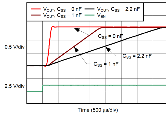
Figure 7-3. Turn-On Response
