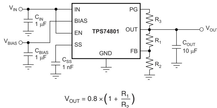
Figure 7-1. Typical Application Circuit for the TPS74801-Q1 (Adjustable)
