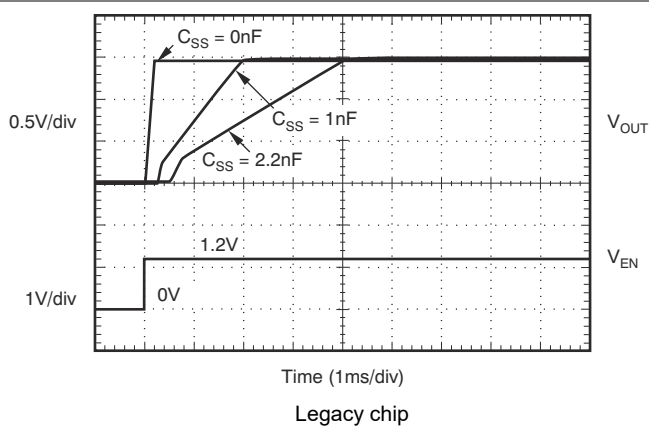
Figure 5-38. Turn-On Response
