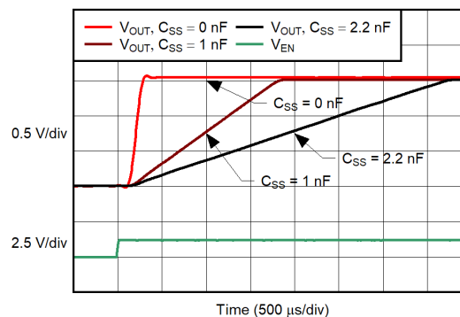
Turn-On Response
