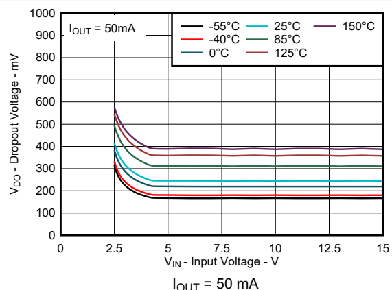
Figure 6-12. TPS71501 Dropout Voltage vs Input Voltage for New Chip
