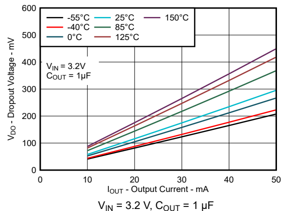
Figure 6-10. Dropout Voltage vs Output Current for New Chip
