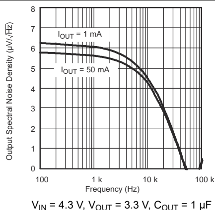
Figure 6-7. Output Spectral Noise Density vs Frequency for Legacy Chip
