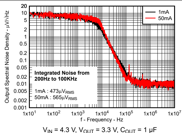
Figure 6-8. Output Spectral Noise Density vs Frequency for New Chip
