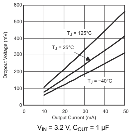
Figure 6-9. Dropout Voltage vs Output Current for Legacy Chip
