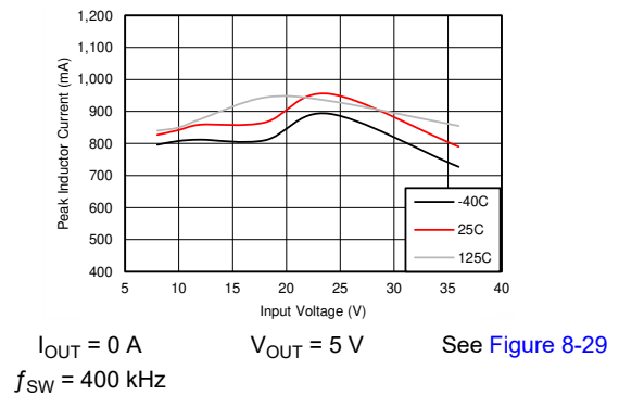
Figure 6-6. I_{PEAK-MIN}
