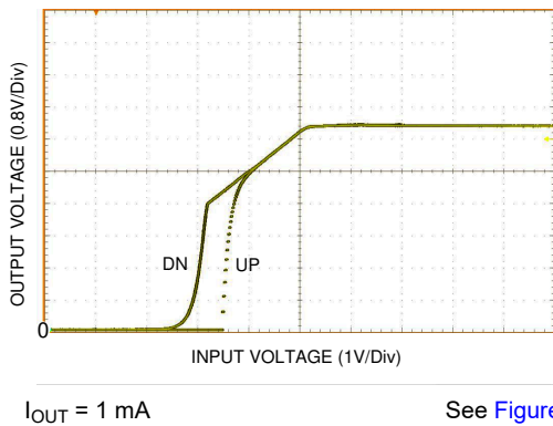
Figure 6-5. UVLO Thresholds
