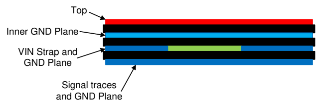
Figure 10-2. Example Layout for VQFN Package
