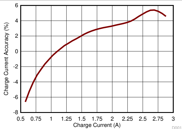
Figure 8-4. Charge Current Accuracy
