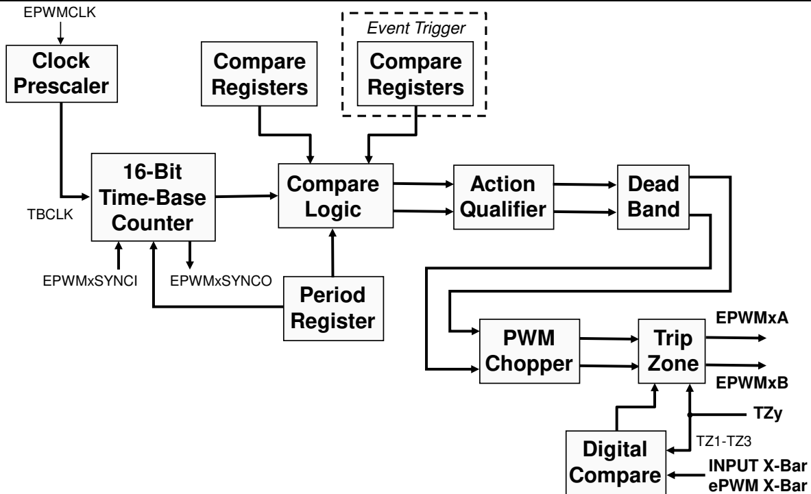
Figure 1-1. Enhanced Pulse Width Modulator (ePWM) Module Block Diagram
