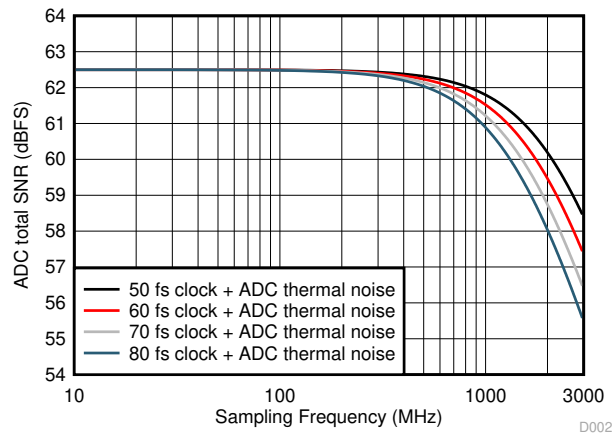
Figure 1-2. Impact of Different Clock Jitter to Total SNR
