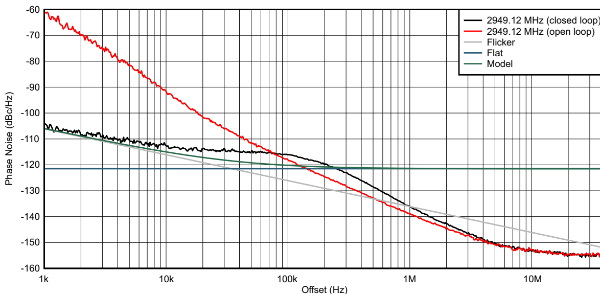
Figure 3-1. Sampling Clock of 2949.12 MHz With 58 fs Jitter
