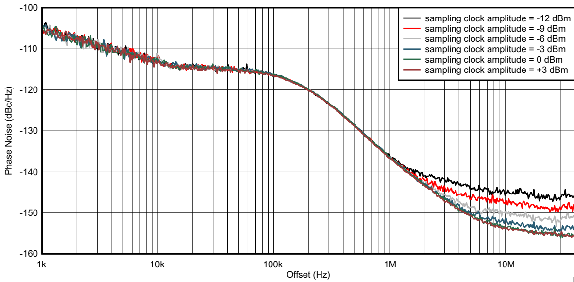
Figure 4-2. Sampling Clock Amplitude
