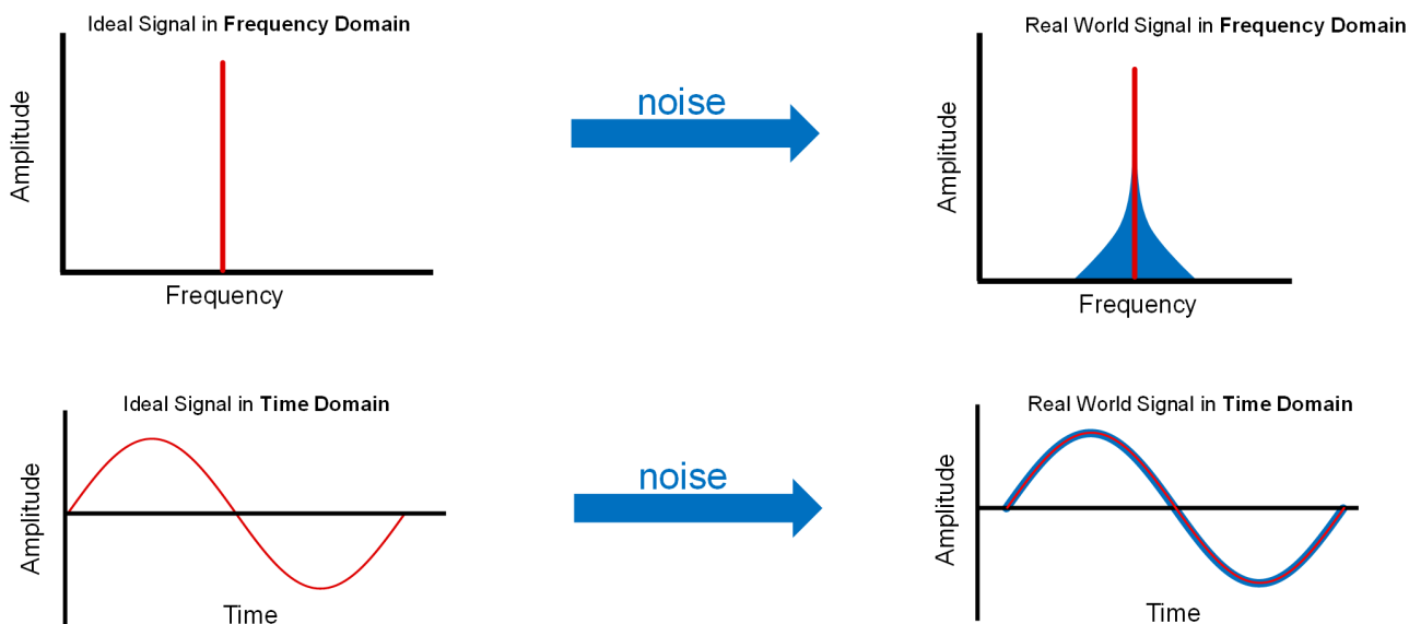
Figure 2-1. Phase Noise in the Frequency and Time Domain
