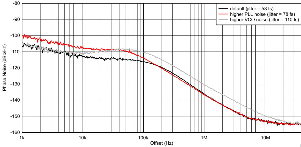
Figure 4-1. Phase Noise Contribution from PLL and VCO
