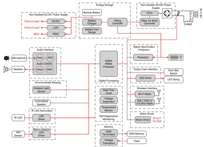
Figure 1. Video Doorbell Block Diagram Example
