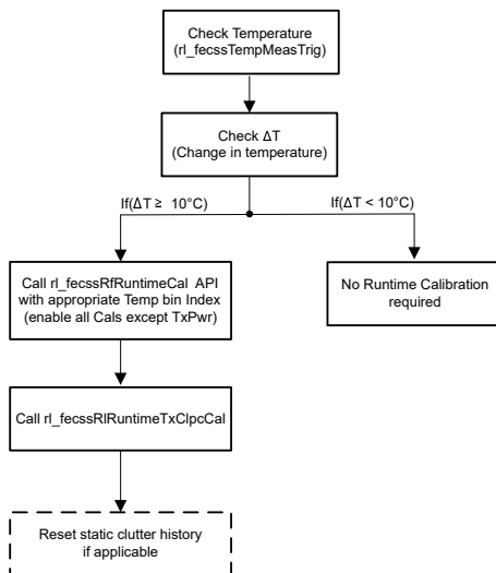
Figure 7-4. In-Field Runtime Calibration Sequence for Applications With TX CLPC Cal
