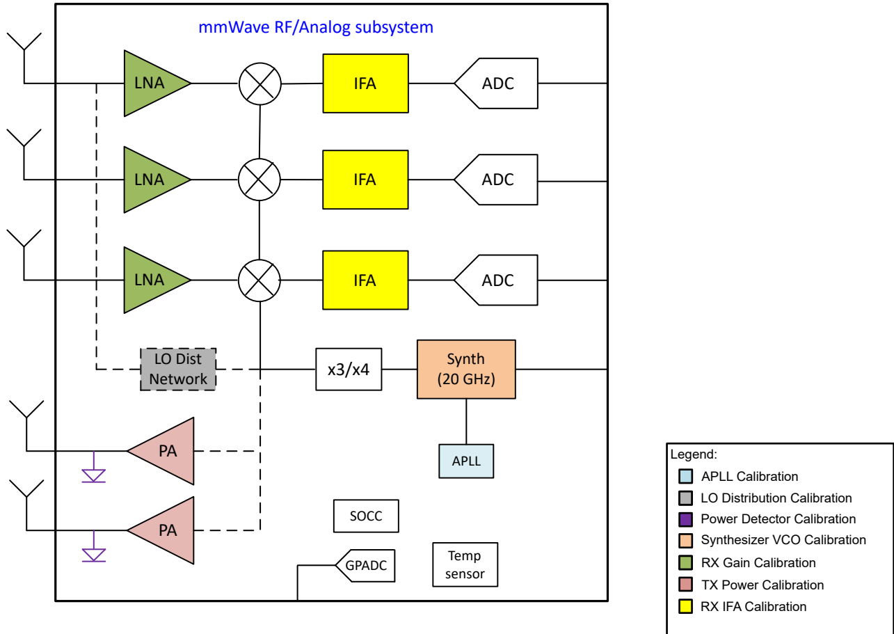
Figure 2-1. mmWave Front-End Architecture
