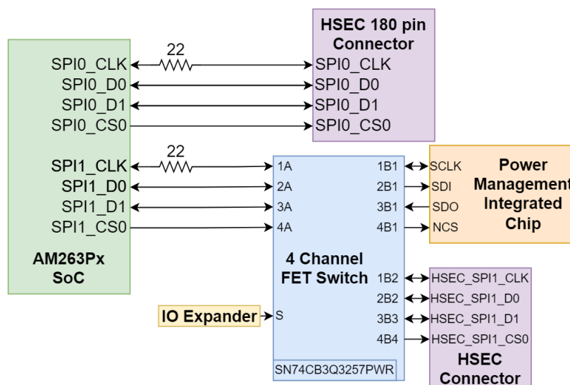
Figure 2-25. SPI
