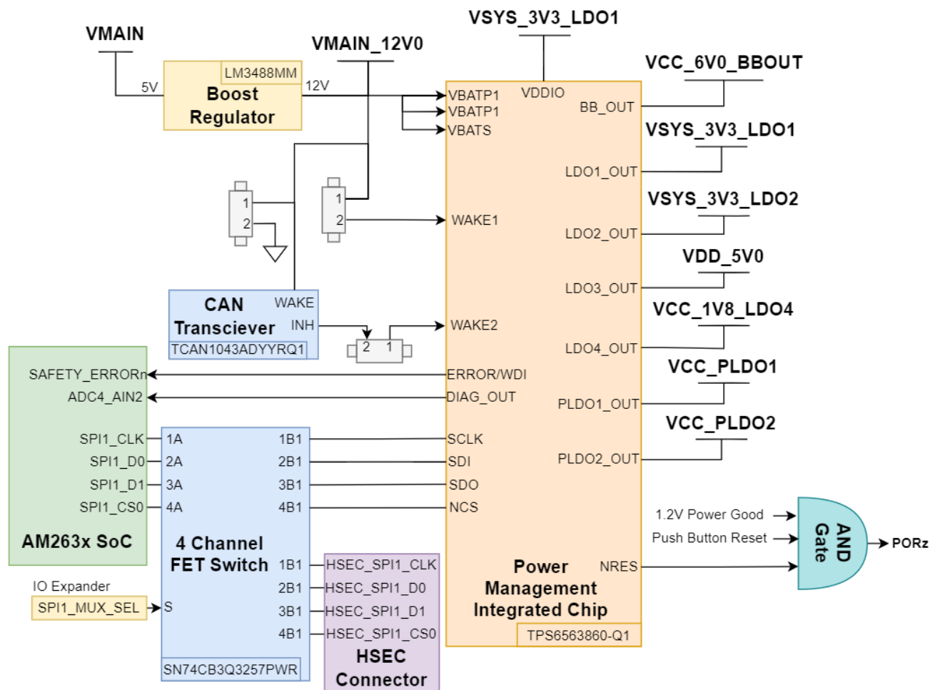
Figure 2-8. PMIC
