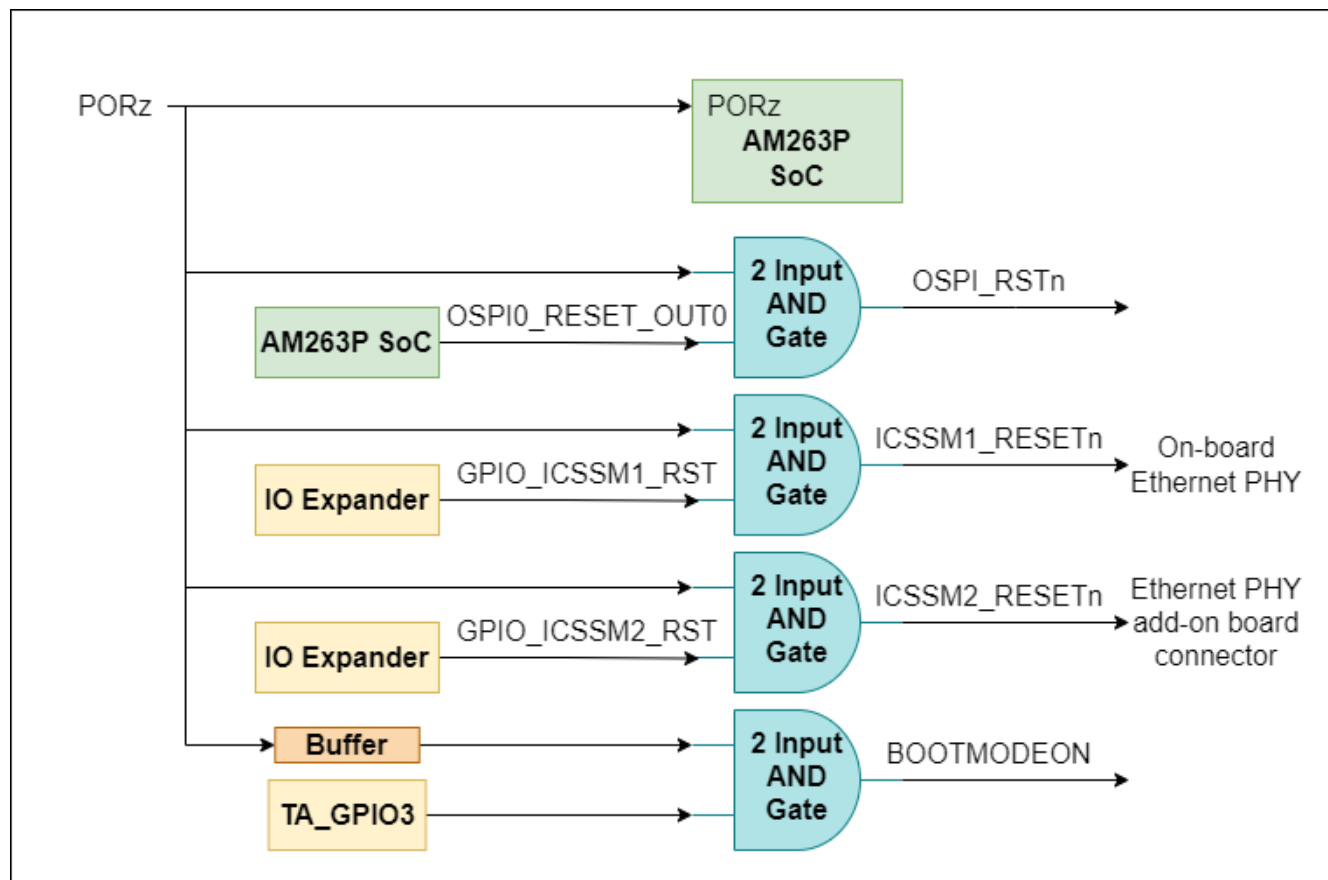
Figure 2-11. PORz Reset Signal Tree
