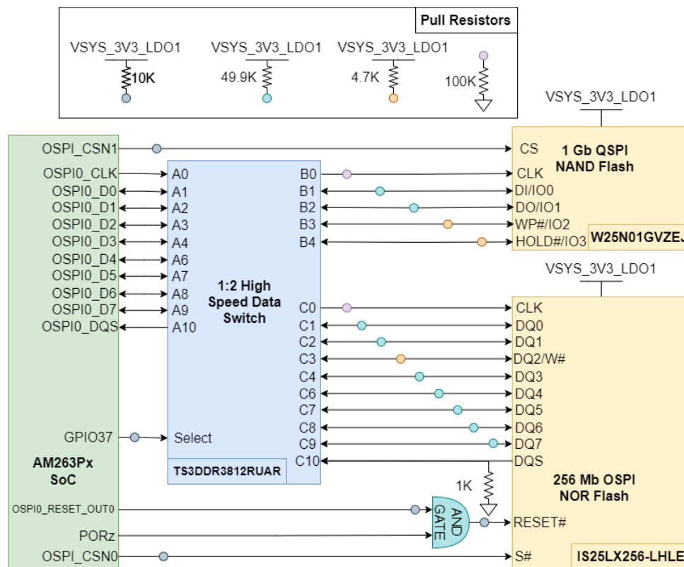
Figure 2-18. OSPI/QSPI Interface
