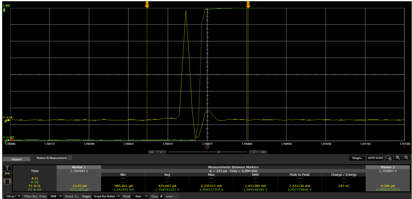
Figure 2-6. 100Hz Pin Wake Up Test Case in 24MHz Mode
