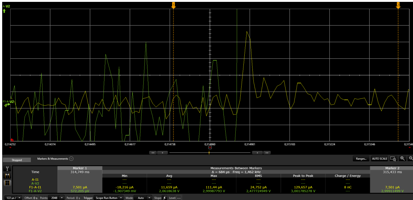
Figure 2-7. 100Hz Pin Wake Up Test Case in 2MHz Mode
