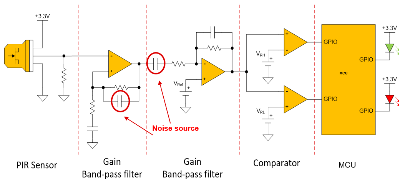
Figure 3-2. PIR Traditional Signal-Chain
