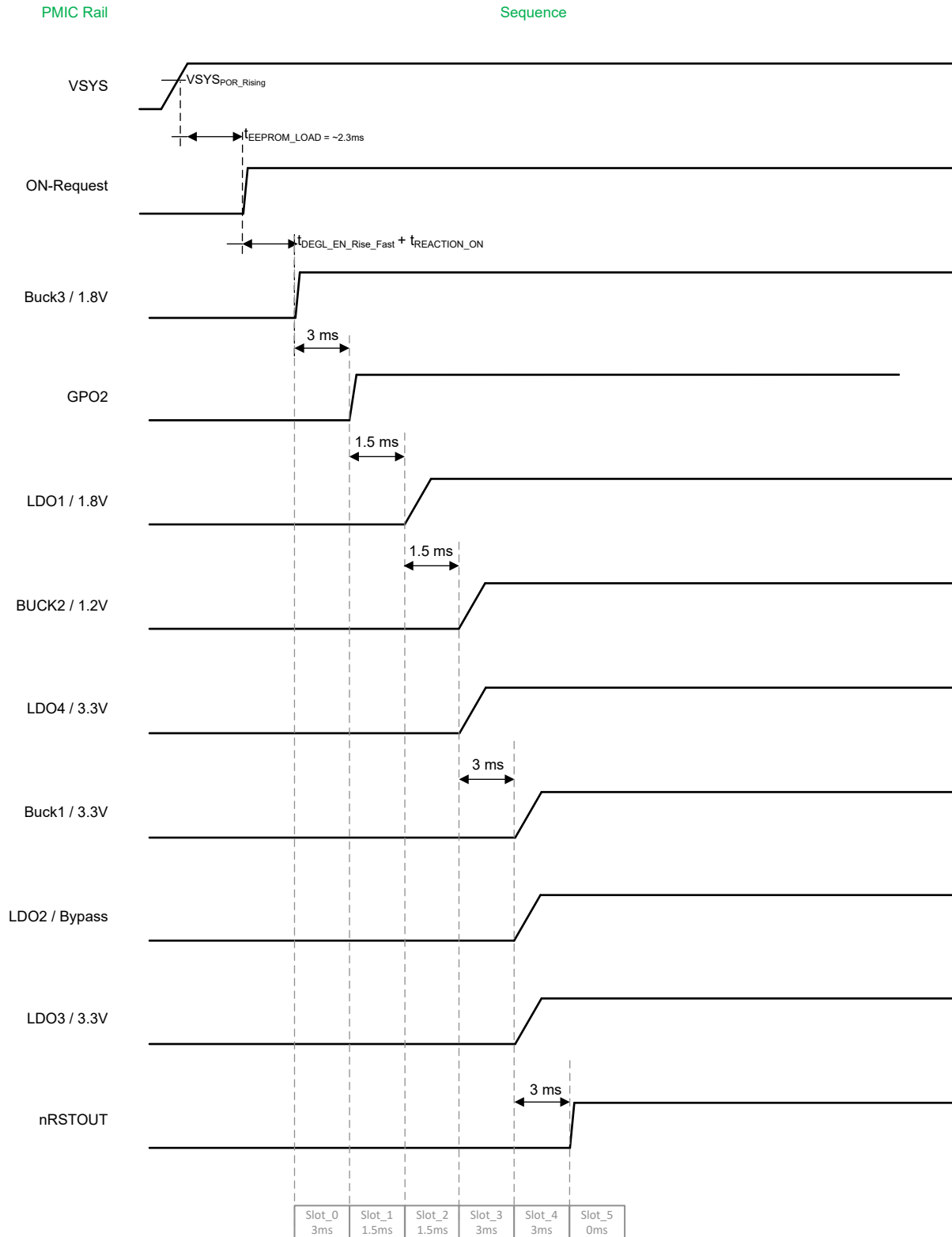
Figure 2-2. TPS6521914 Power-Up Sequence
