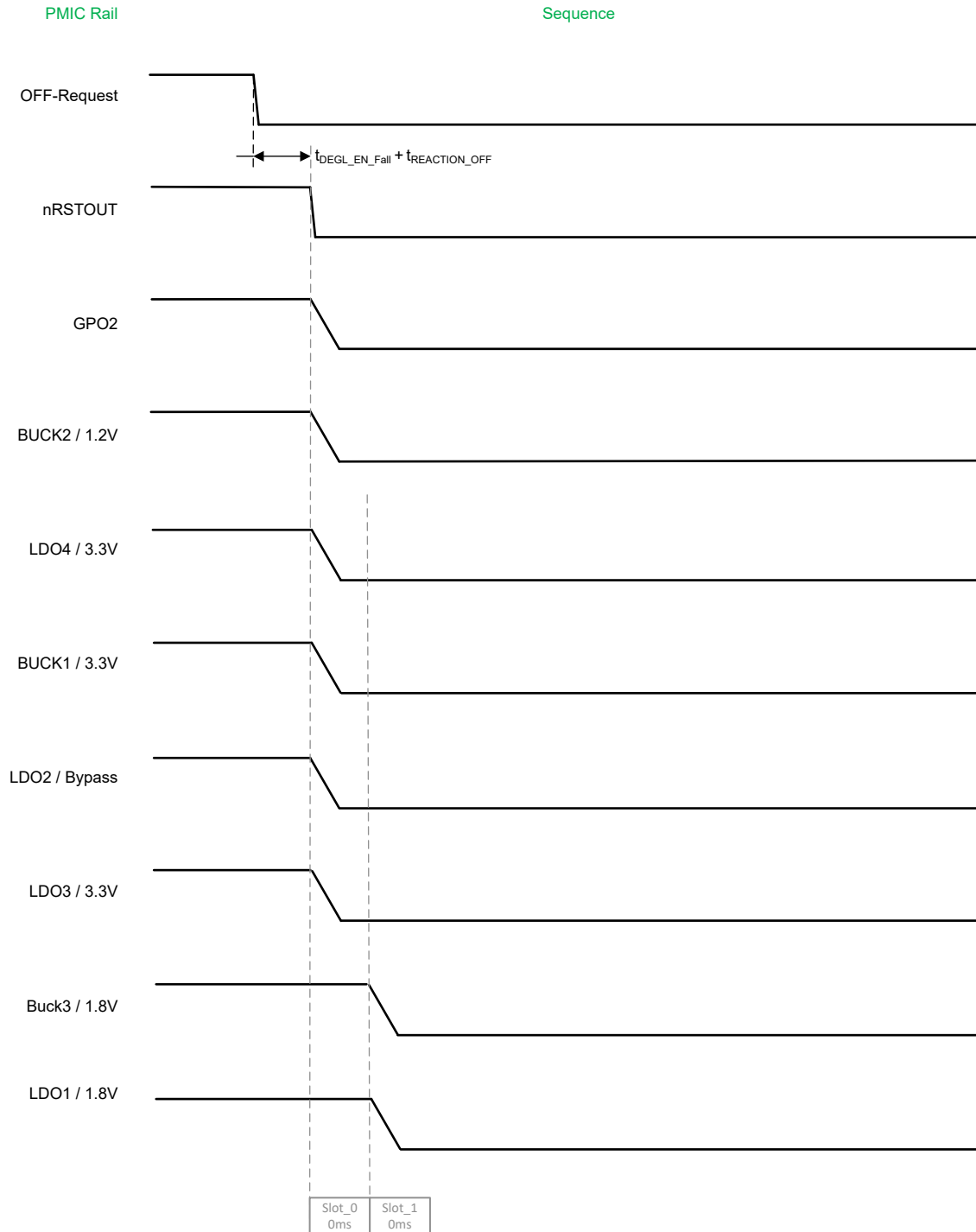
Figure 2-3. TPS6521914 Power-Down Sequence
