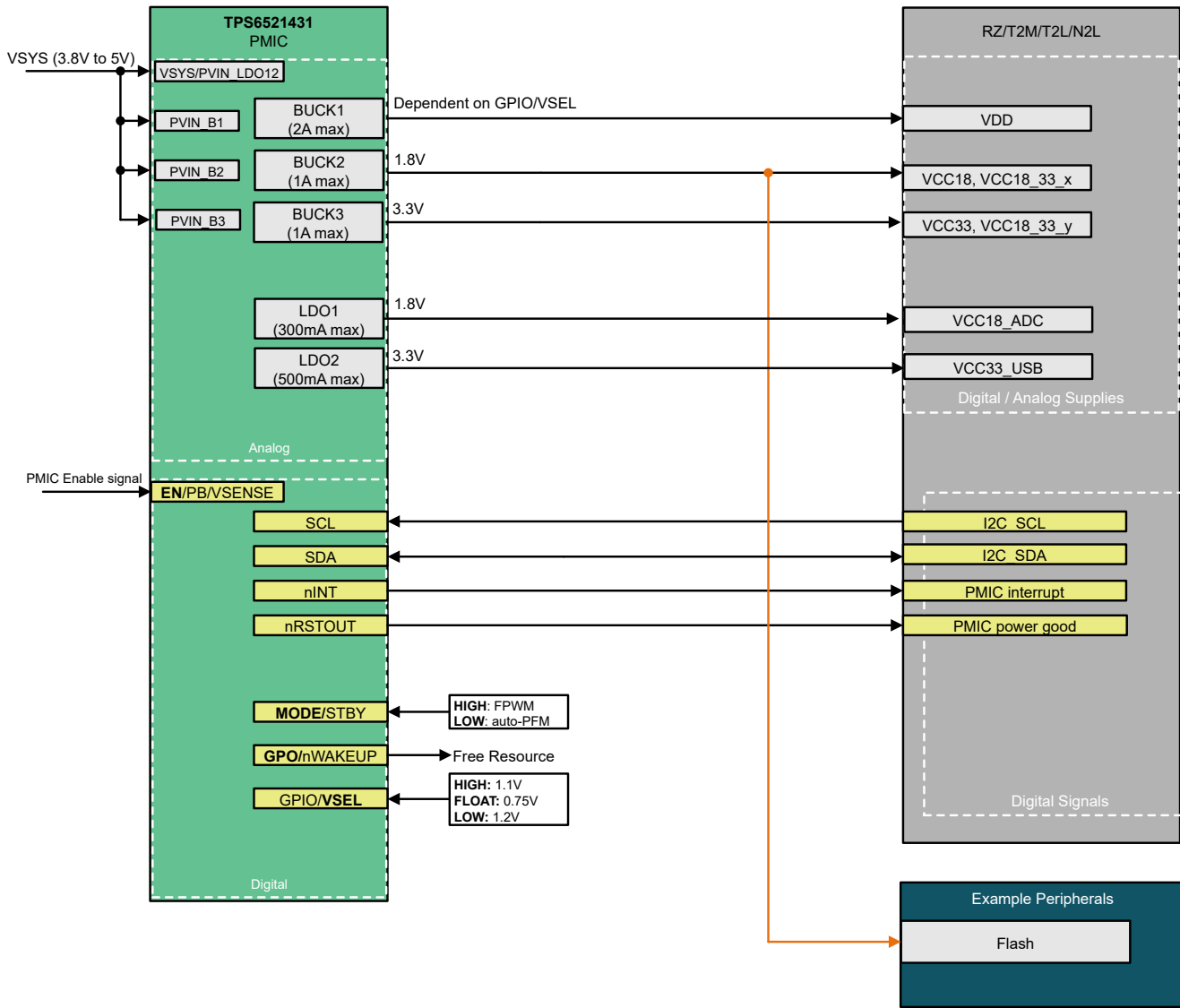
Figure 2-2. TPS6521431 Example Block Diagram
