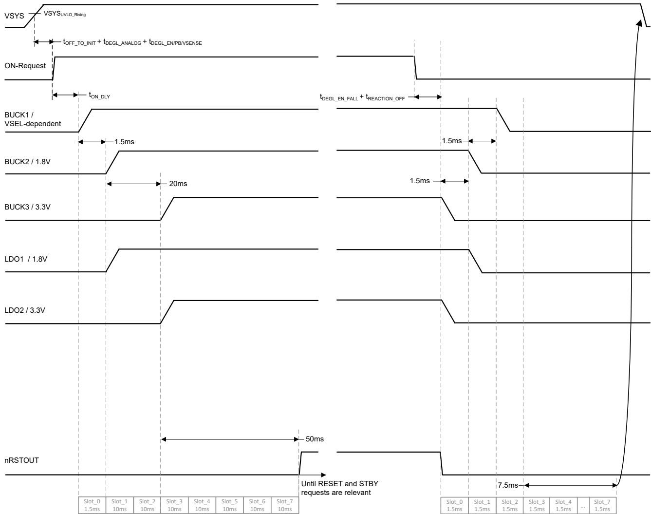
Figure 2-1. TPS6521431 Power Sequence
