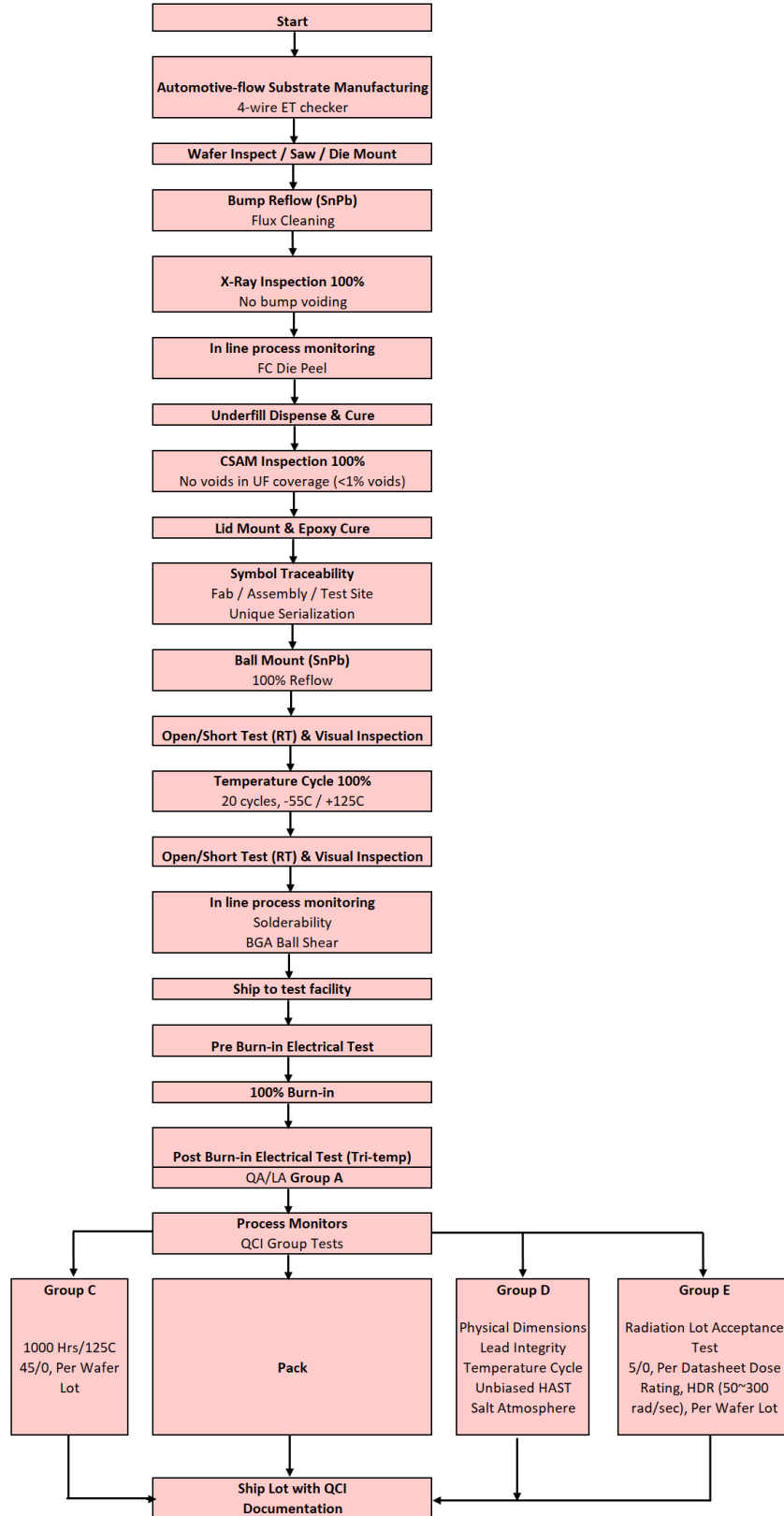
Figure 2-1. ADC12QJ1600-SHP Space High Grade in Plastic Production Flow Chart
