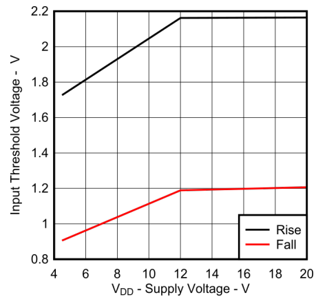
Figure 6-27. Input Threshold vs Supply Voltage
