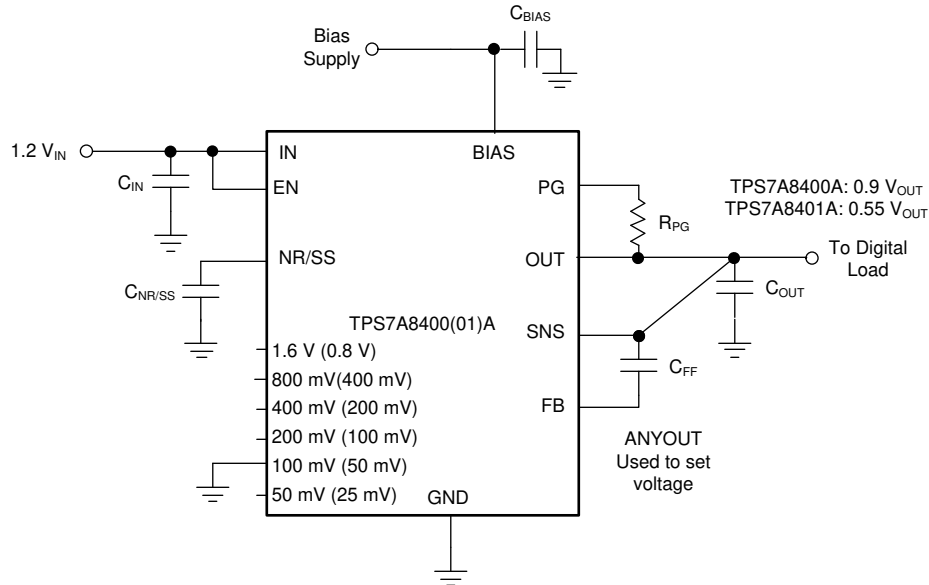
Figure 8-21. TPS7A84A Typical Application
