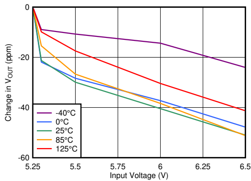
Figure 6-31. Line Regulation vs V_{IN} (5-V Output)
