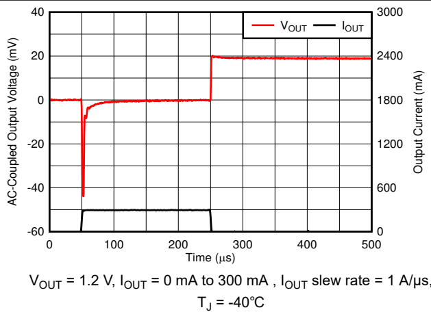
Figure 6-51. Load Transient
