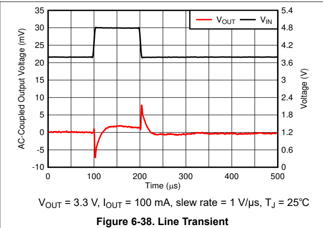
Figure 6-38. Line Transient
