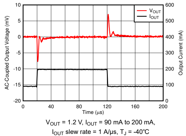
Figure 6-54. Load Transient
