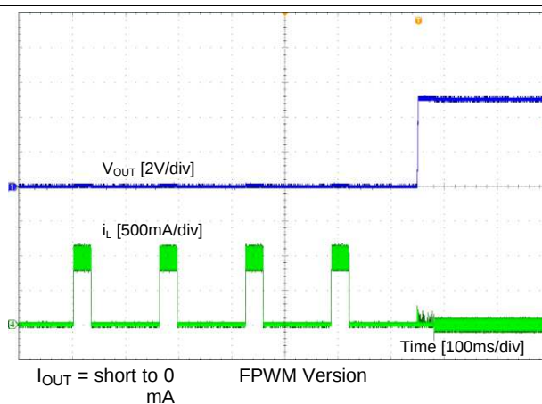
Figure 26. Short Recovery
