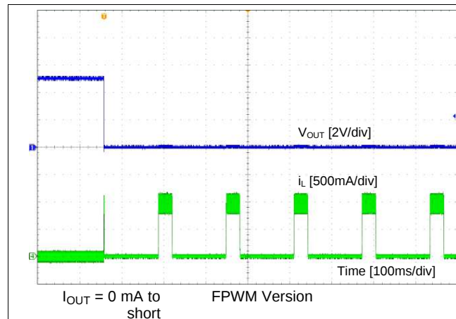
Figure 25. Short Protection
