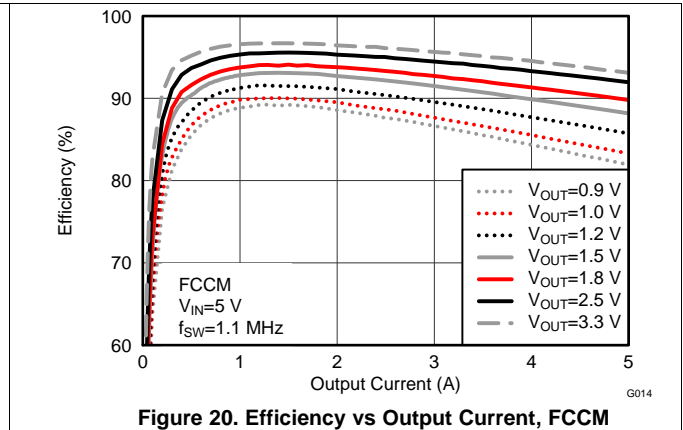
Figure 20. Efficiency vs Output Current, FCCM
