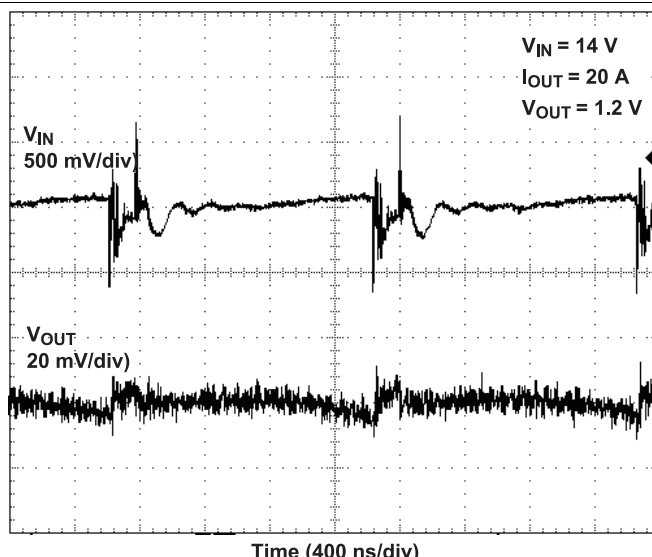
Figure 26. Ripple Waveform
