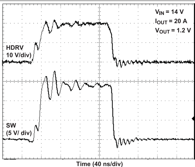
Figure 25. Switching Waveform
