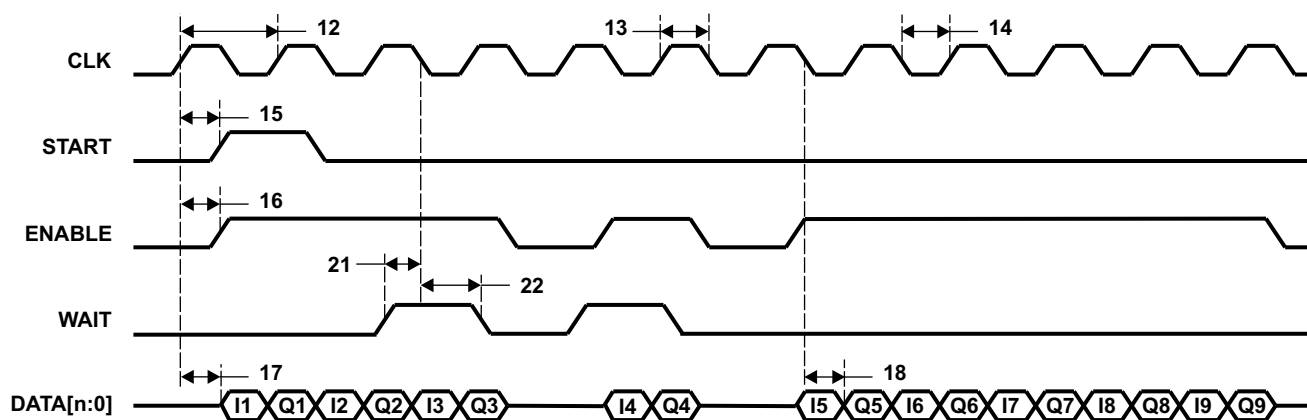
Figure 4-83. uPP Double Data Rate (DDR) Transmit Timing
