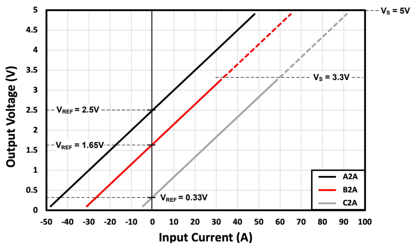
Figure 8-5. Output Voltage Relationship to Input Current for TMCS11xxx2A-Q1
