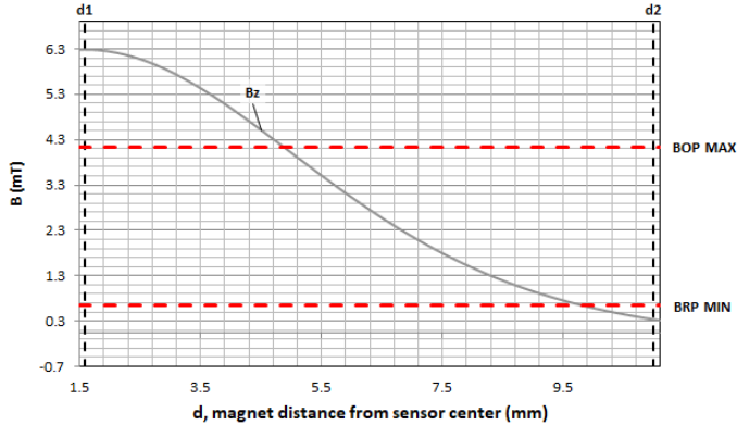
Figure 9-12. B-Field Hypothesis
