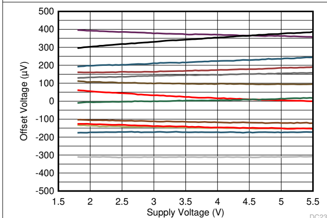
Figure 6-5. Offset Voltage vs Power Supply
