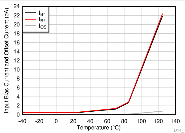
Figure 6-8. I_B and I_{OS} vs Temperature
