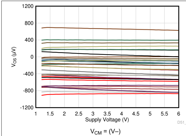
Figure 6-7. Offset Voltage vs Supply Voltage
