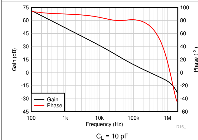
Figure 6-11. Open-Loop Gain and Phase vs Frequency
