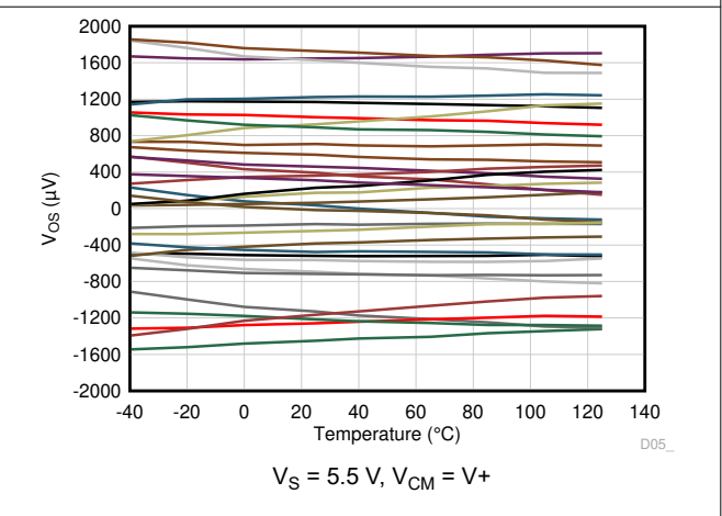
Figure 6-4. Input Offset Voltage vs Temperature
