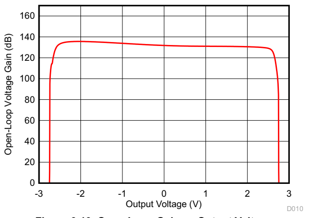
Figure 6-10. Open-Loop Voltage Gain vs Output Voltage
