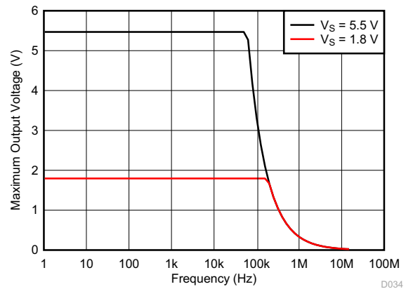
Figure 6-34. Maximum Output Voltage vs Frequency
