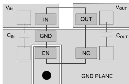
Figure 27. X2SON Layout Example
