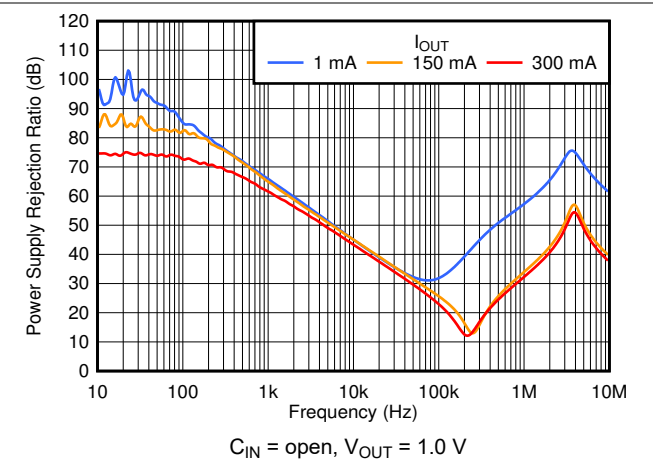
Figure 5-14. PSRR vs Frequency and I_{OUT}
