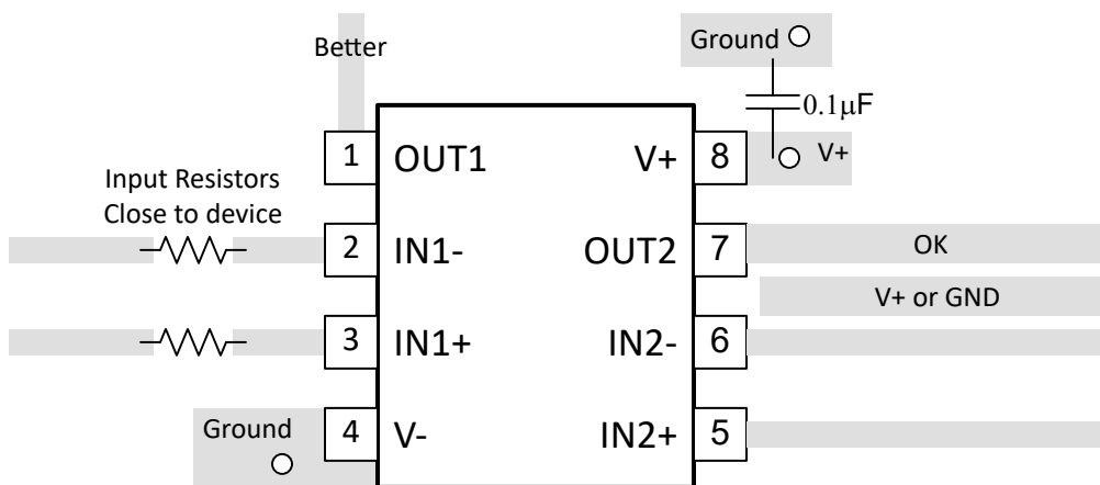
Figure 7-12. Dual Layout Example
