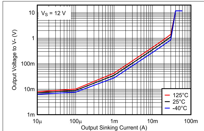
Figure 6-7. Output Voltage vs. Output Sinking Current, 12V
