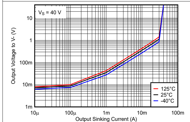
Figure 6-9. Output Voltage vs. Output Sinking Current, 40V
