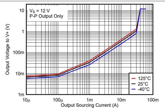
Figure 6-8. Output Voltage vs. Output Sourcing Current, 12V
