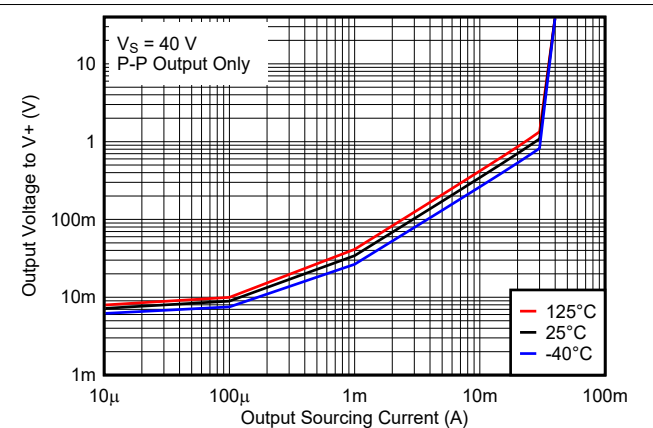
Figure 6-10. Output Voltage vs. Output Sourcing Current, 40V
