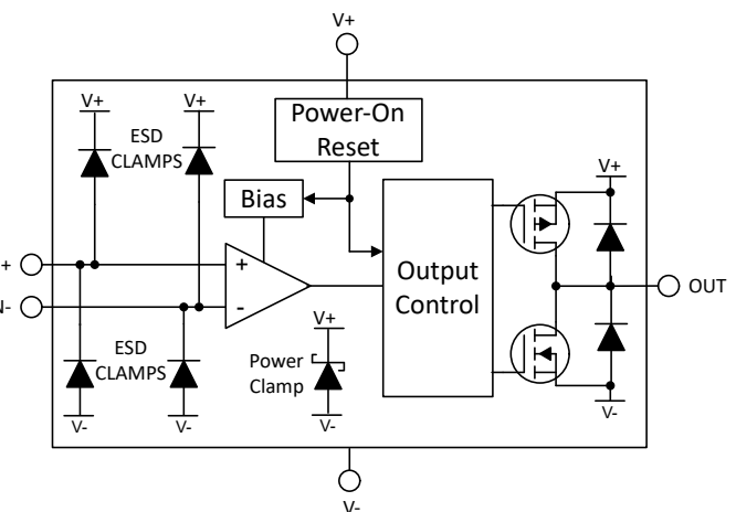
Figure 7-2. TLV181x-Q1 Push-Pull Block Diagram
