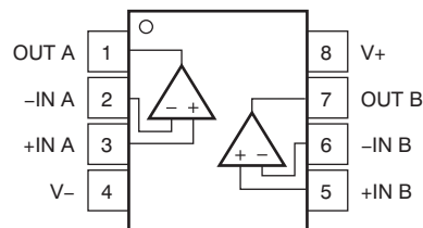
Pin Functions: TLV2171
