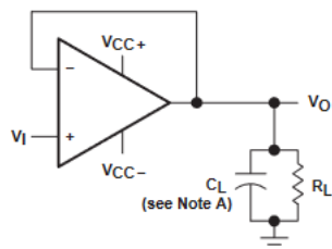
Figure 6-1. Slew-Rate Test Circuit
