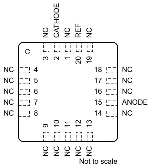
Figure 4-4. FK Package 20-Pin LCCC Top View
