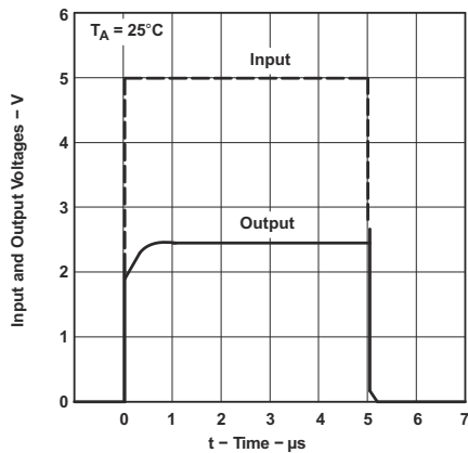
Figure 5-11. Pulse Response
