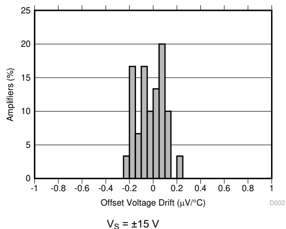
Figure 6-3. Input Offset Voltage Drift Histogram
