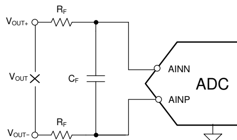
Figure 9-9. Differential Filter
