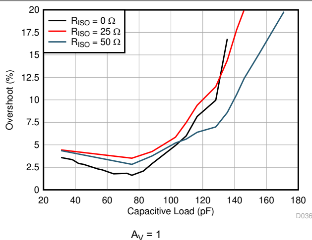
Figure 6-25. Small-Signal Overshoot vs Capacitive Load
