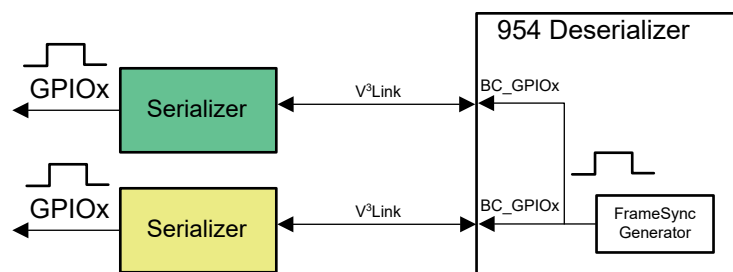
Figure 7-18. Internal FrameSync
