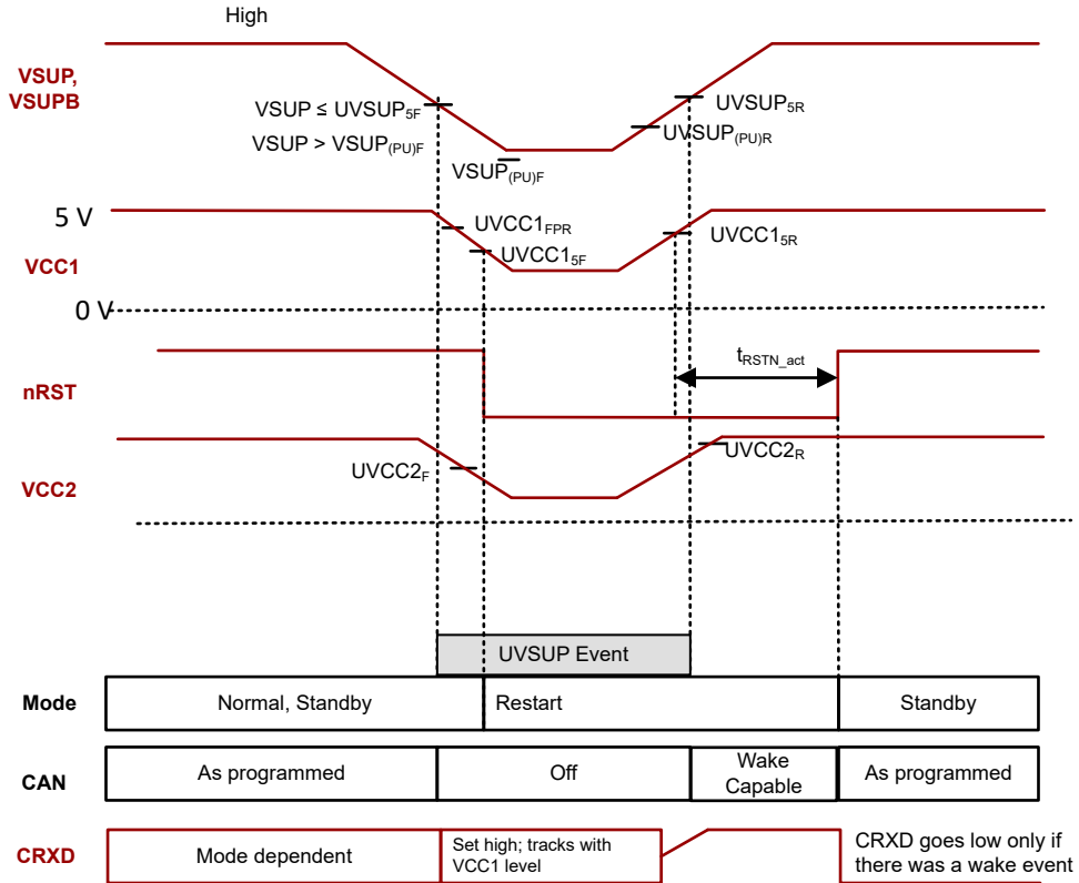
Figure 10-3. Brownout Above VSUP_{(PI)F} for VCC1 = 5V
