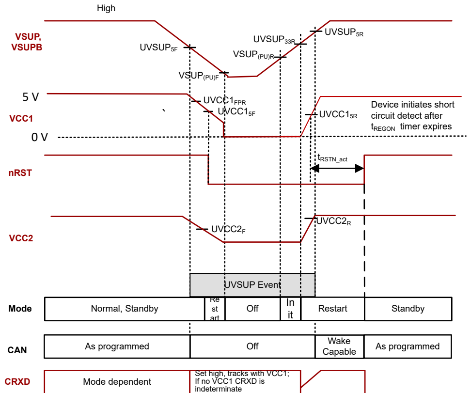
Figure 10-4. Brownout Below VSUP_{(PI)F}
