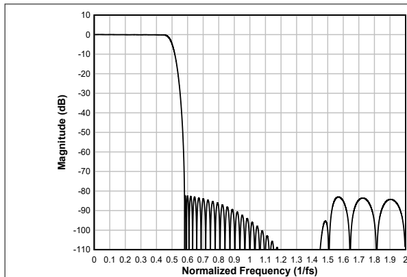
Figure 6-75. Linear-phase Interpolation Filter Magnitude Response
