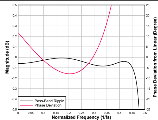
Figure 6-98. Ultra-Low-Latency interpolation Filter Pass-Band Ripple and Phase Deviation
