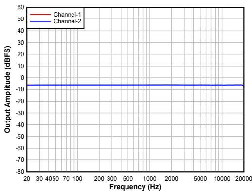
AC-coupled differential line input (-6dBFS)
