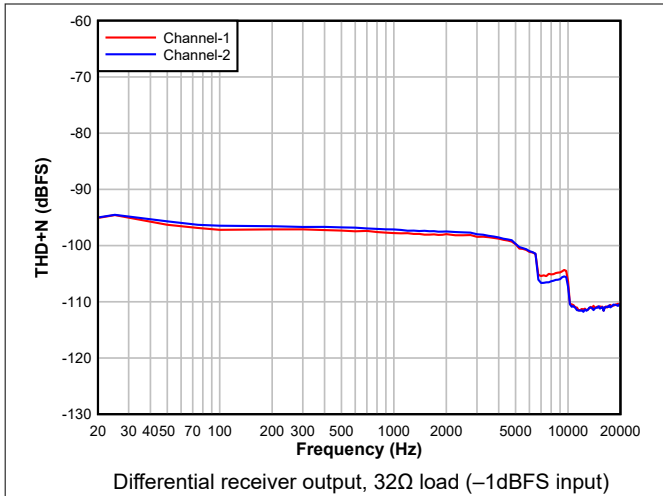
Figure 5-27. DAC THD+N Level vs Frequency
