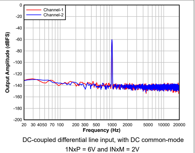
Figure 8-5. ADC FFT with -60dBFS Input
