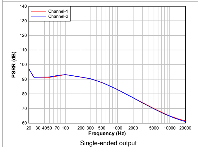
Figure 5-33. DAC PSRR vs Frequency
