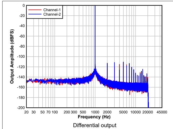
Figure 5-31. DAC FFT with -1dBFS Input
