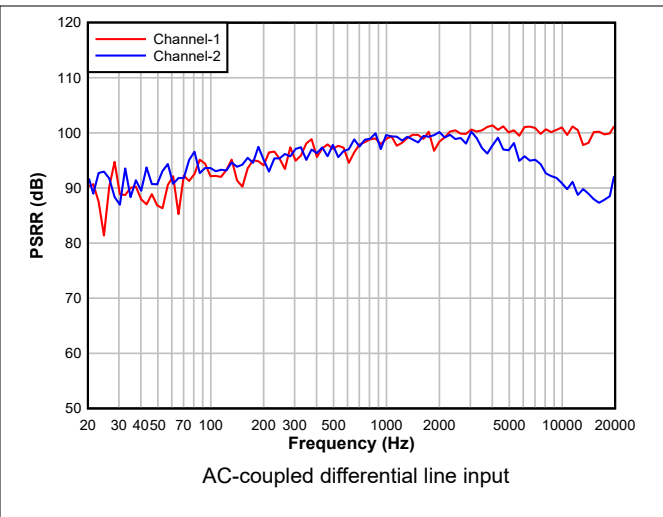
Figure 5-16. ADC PSRR vs Frequency
