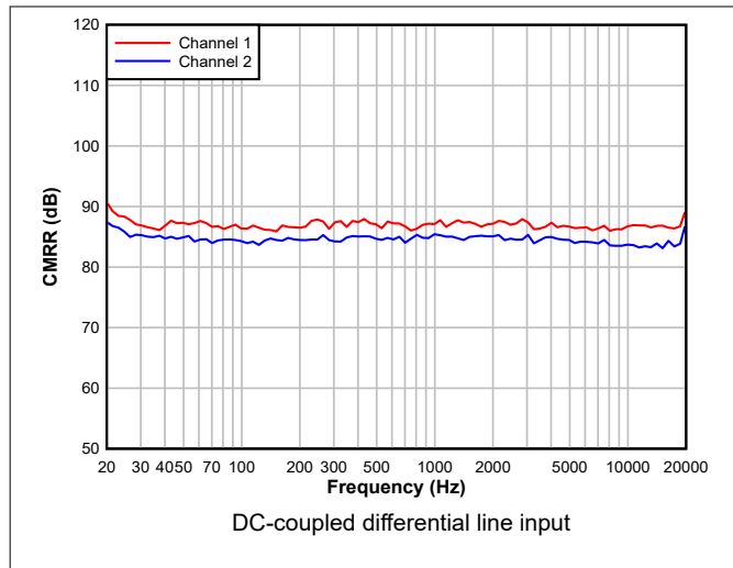
Figure 5-15. ADC CMRR vs Frequency
