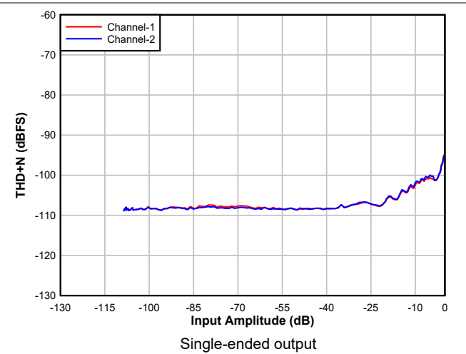
Figure 5-20. DAC THD+N Level vs Input
