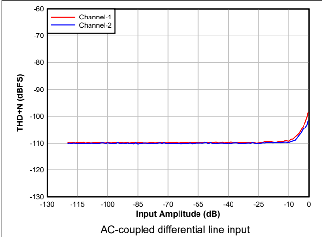
Figure 8-2. ADC THD+N Level vs Input
