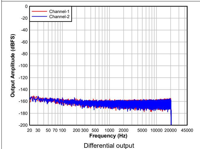
Figure 5-29. DAC FFT with Idle Channel Input
