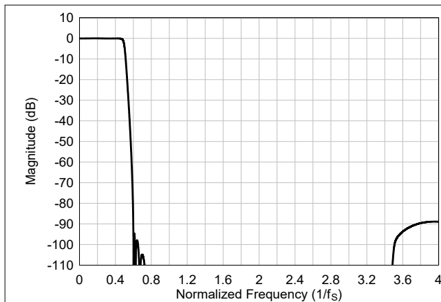
Figure 6-97. Ultra-Low-Latency interpolation Filter Magnitude Response
