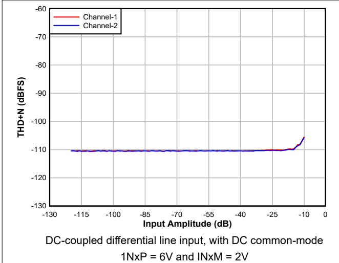
Figure 8-4. ADC THD+N Level vs Input
