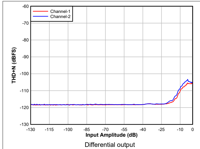
Figure 5-19. DAC THD+N Level vs Input
