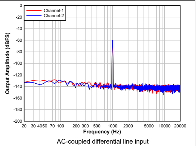
Figure 8-3. ADC FFT with -60dBFS Input
