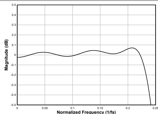
Figure 6-38. Linear-phase Decimation Filter Pass-Band Ripple
