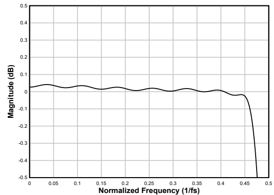
Figure 6-26. Linear-phase Decimation Filter Pass-Band Ripple
