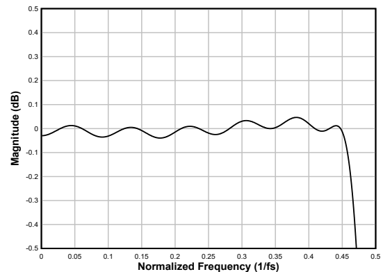
Figure 6-28. Linear-phase Decimation Filter Pass-Band Ripple
