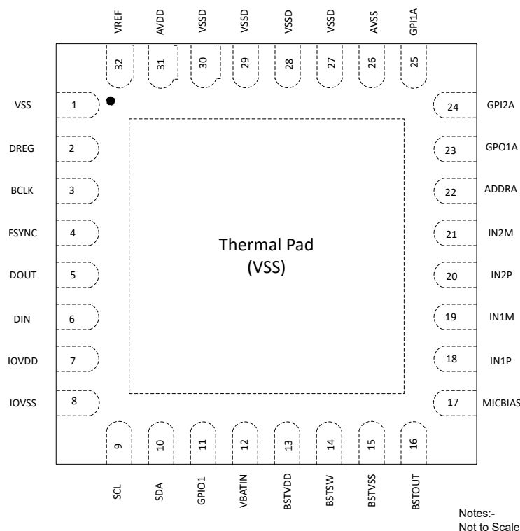
Figure 4-1. TAA5412-Q1 RTV Package, 32-Pin WQFN With Exposed Thermal Pad, Top View
