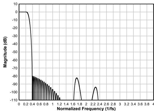
Figure 6-35. Linear-phase Decimation Filter Magnitude Response
