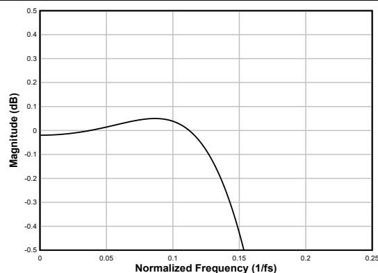
Figure 6-40. Linear-phase Decimation Filter Pass-Band Ripple
