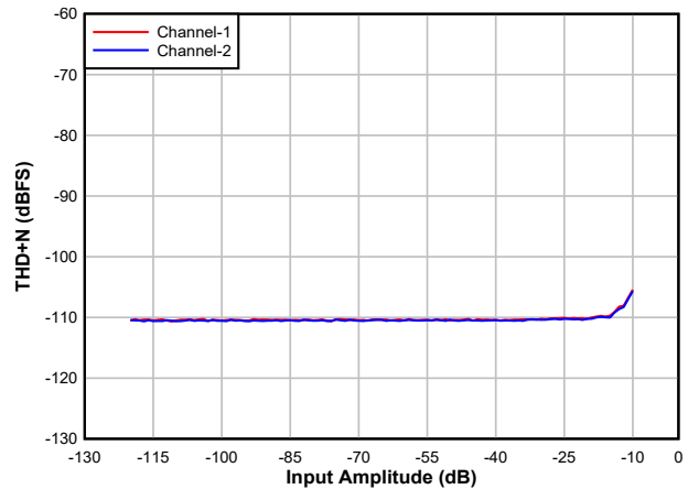
Figure 8-5. ADC THD+N Level vs Input
