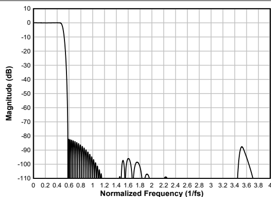
Figure 6-31. Linear-phase Decimation Filter Magnitude Response
