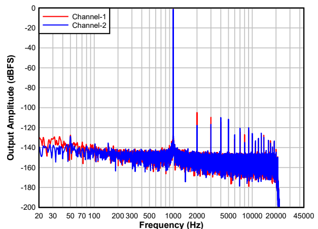
Figure 5-14. ADC FFT with -1dBFS Input
