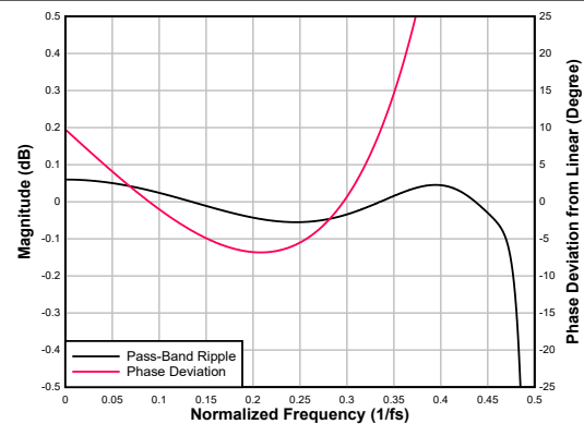
Figure 6-60. Ultra Low-latency Decimation Filter Pass-Band Ripple and Phase Deviation
