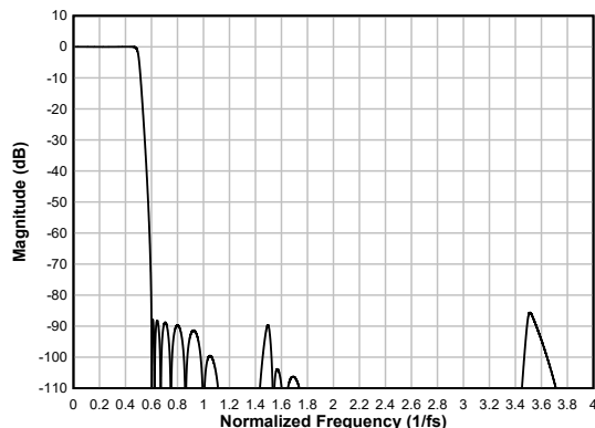
Figure 6-47. Low-latency Decimation Filter Magnitude Response
