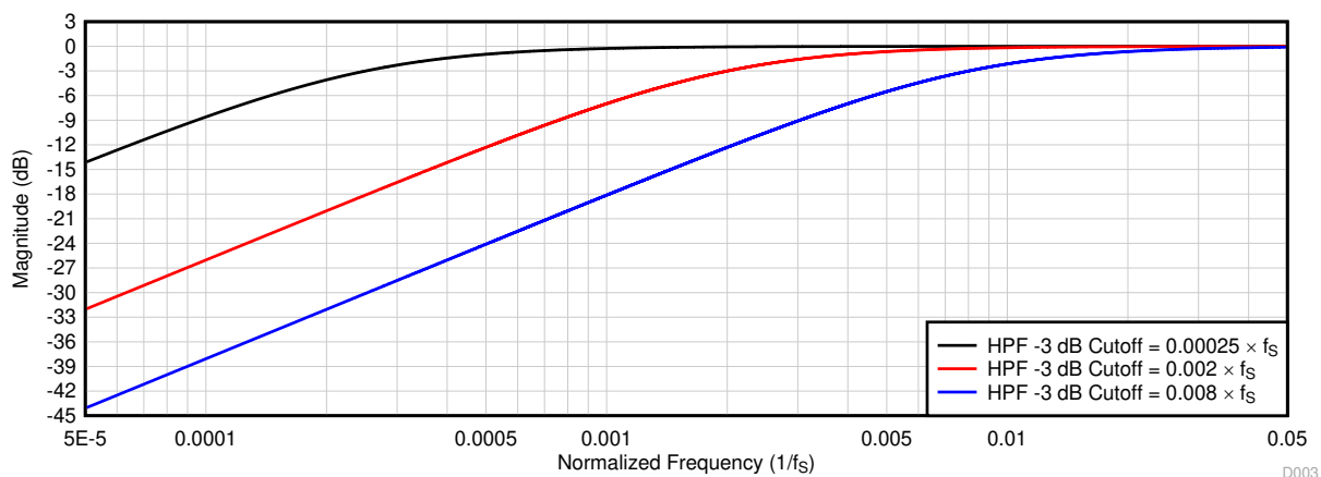
Figure 6-21. HPF Filter Frequency Response Plot
