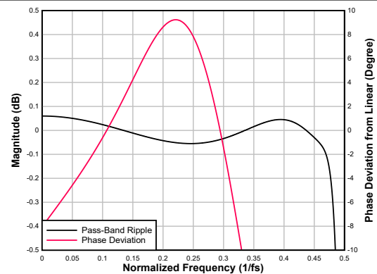
Figure 6-50. Low-latency Decimation Filter Pass-Band Ripple and Phase Deviation
