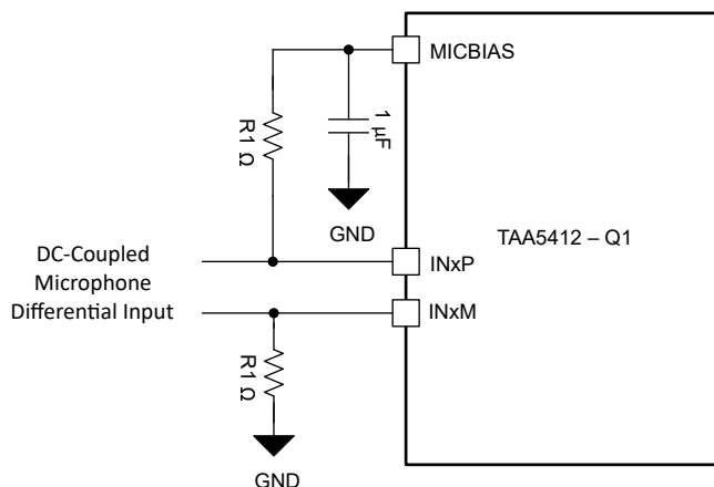
Figure 6-14. DC-Coupled Microphone Differential Input Connection
