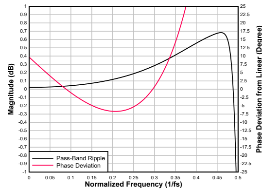
Figure 6-52. Ultra Low-latency Decimation Filter Pass-Band Ripple and Phase Deviation
