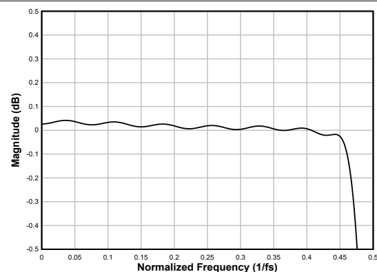
Figure 6-24. Linear-phase Decimation Filter Pass-Band Ripple
