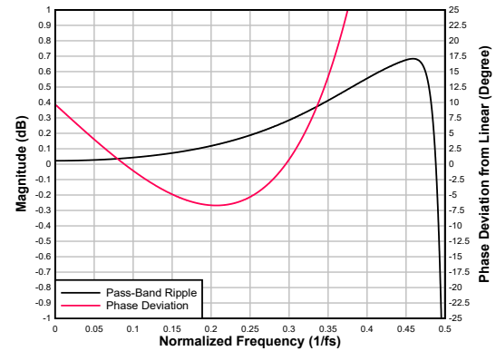
Figure 6-54. Ultra Low-latency Decimation Filter Pass-Band Ripple and Phase Deviation
