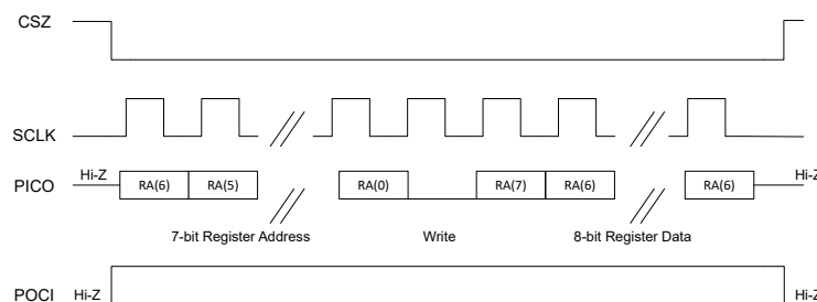
Figure 6-67. SPI Single-Byte Write Transfer
