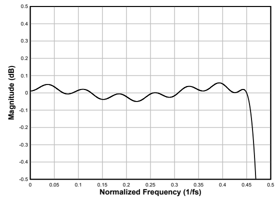
Figure 6-34. Linear-phase Decimation Filter Pass-Band Ripple
