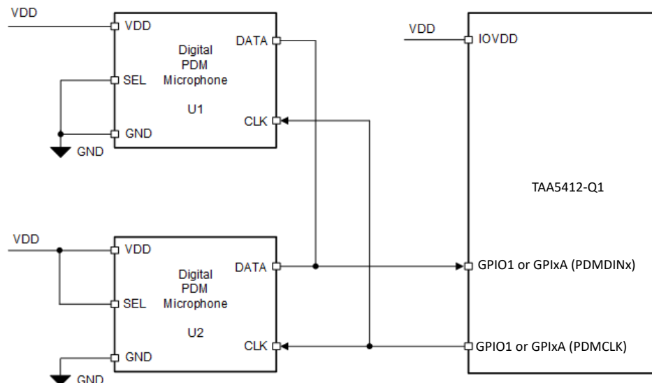
Figure 6-18. Digital PDM Microphones Connection Diagram for the TAA5412-Q1
