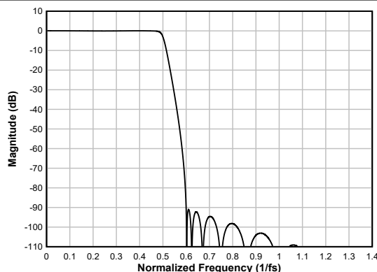
Figure 6-59. Ultra Low-latency Decimation Filter Magnitude Response
