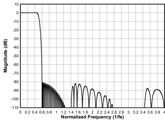
Figure 6-27. Linear-phase Decimation Filter Magnitude Response
