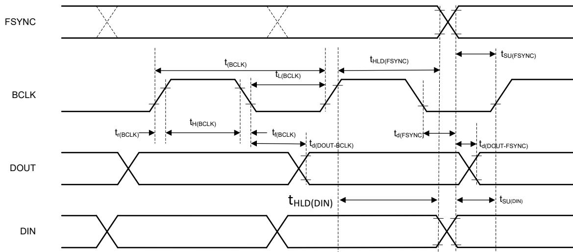
Figure 5-3. TDM, I²S, LJ Interface Timing Diagram
