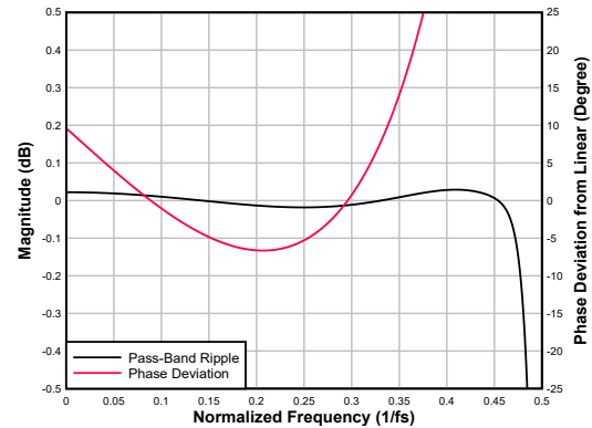
Figure 6-58. Ultra Low-latency Decimation Filter Pass-Band Ripple and Phase Deviation
