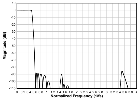
Figure 6-57. Ultra Low-latency Decimation Filter Magnitude Response
