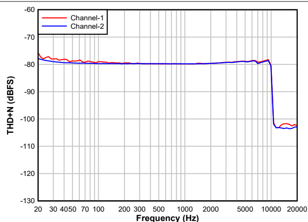
Figure 5-10. ADC THD+N vs Frequency
