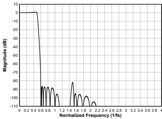
Figure 6-51. Ultra Low-latency Decimation Filter Magnitude Response
