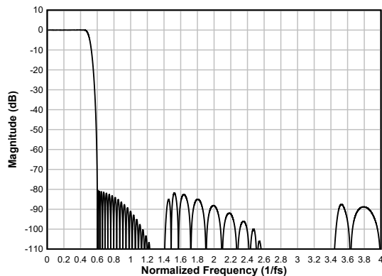
Figure 6-29. Linear-phase Decimation Filter Magnitude Response
