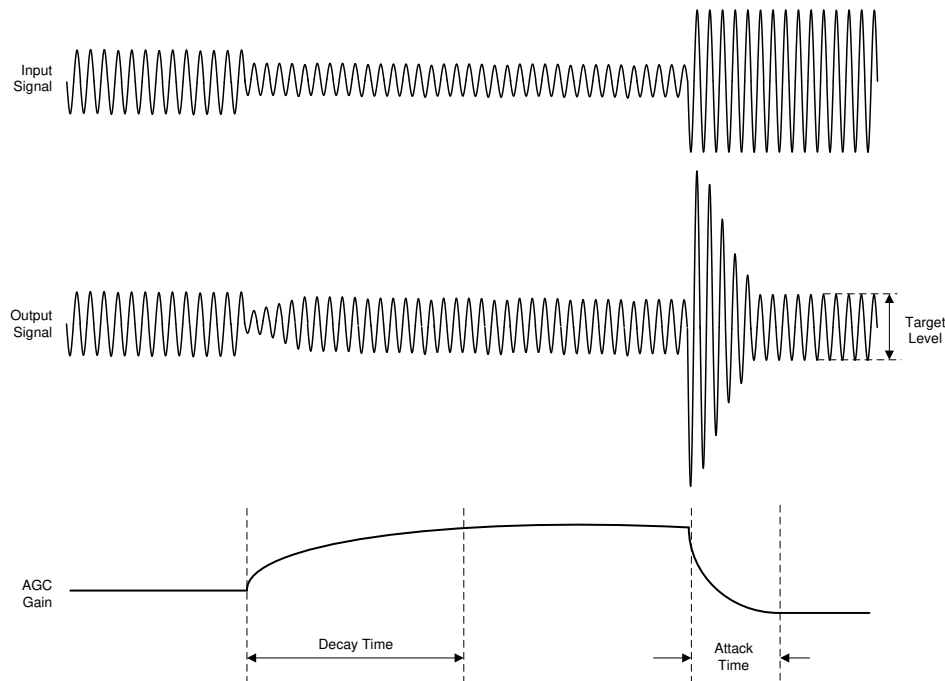
Figure 6-61. AGC Characteristics
