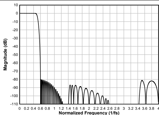
Figure 6-23. Linear-phase Decimation Filter Magnitude Response
