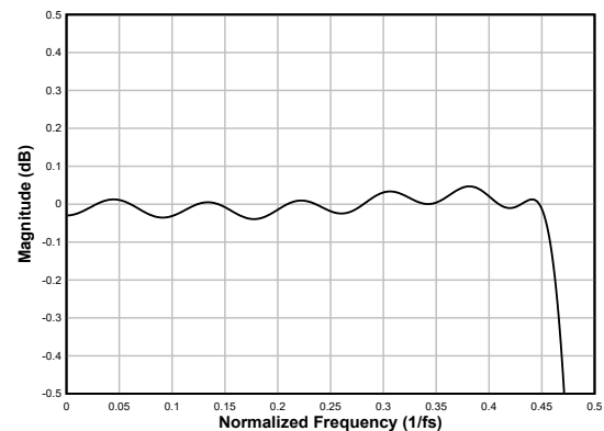
Figure 6-30. Linear-phase Decimation Filter Pass-Band Ripple
