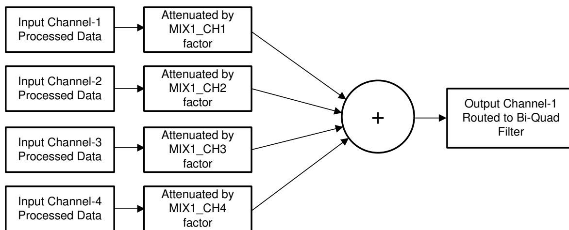
Figure 6-22. Programmable Digital Mixer Block Diagram
