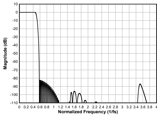
Figure 6-33. Linear-phase Decimation Filter Magnitude Response
