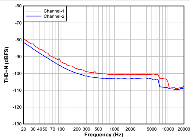
Figure 5-9. ADC THD+N vs Frequency
