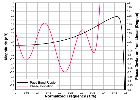
Figure 6-44. Low-latency Decimation Filter Pass-Band Ripple and Phase Deviation
