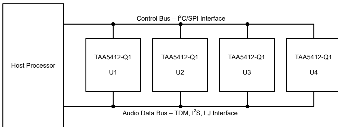
Figure 6-13. Multiple TAA5412-Q1 Devices With Shared Control and Audio Data Buses
