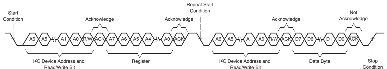
Figure 6-65. I 2 C Single-Byte Read Transfer
