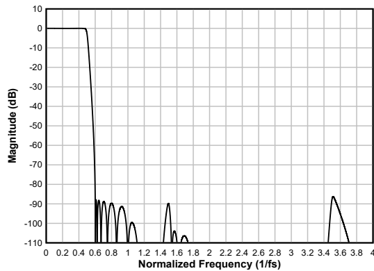
Figure 6-45. Low-latency Decimation Filter Magnitude Response
