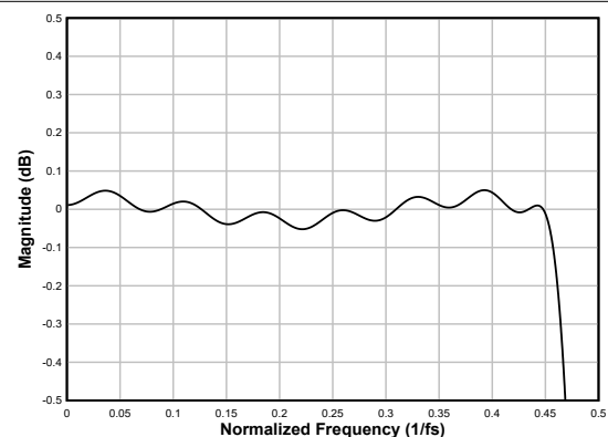
Figure 6-32. Linear-phase Decimation Filter Pass-Band Ripple
