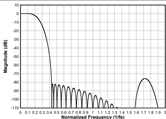
Figure 6-39. Linear-phase Decimation Filter Magnitude Response
