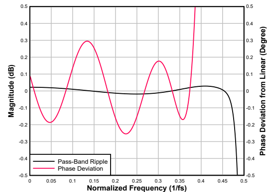
Figure 6-48. Low-latency Decimation Filter Pass-Band Ripple and Phase Deviation
