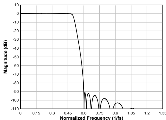
Figure 6-49. Low-latency Decimation Filter Magnitude Response
