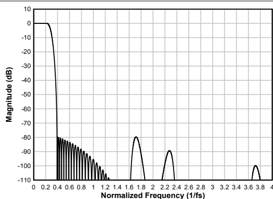
Figure 6-37. Linear-phase Decimation Filter Magnitude Response
