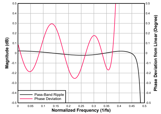
Figure 6-46. Low-latency Decimation Filter Pass-Band Ripple and Phase Deviation
