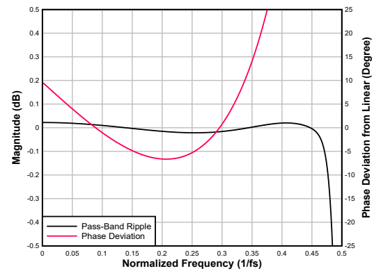
Figure 6-56. Ultra Low-latency Decimation Filter Pass-Band Ripple and Phase Deviation
