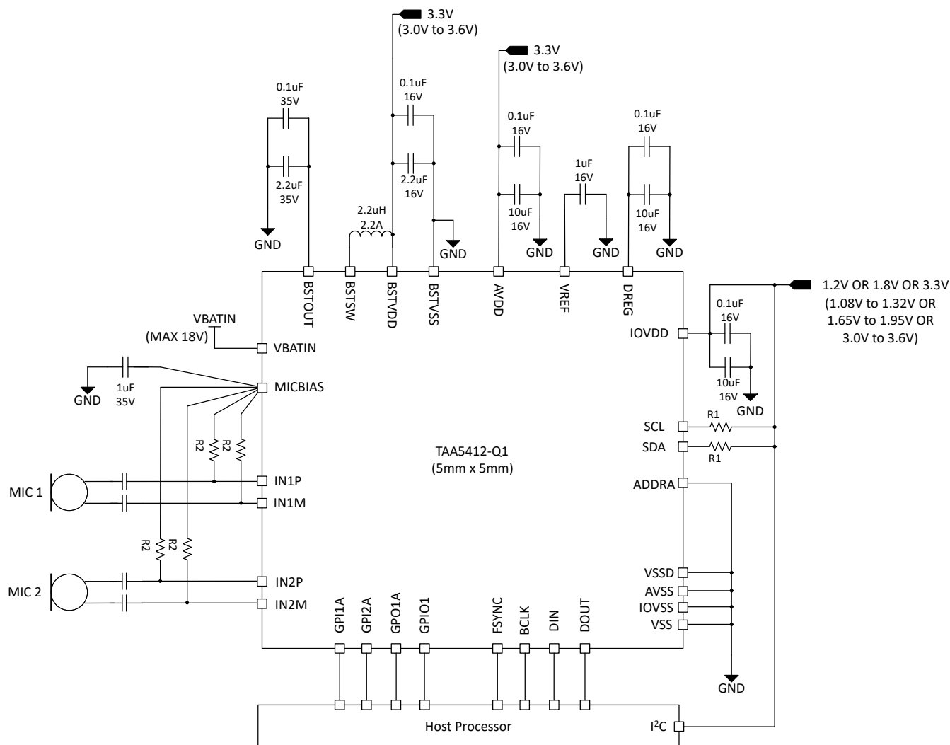
Figure 8-1. Stereo Microphone Block Diagram
