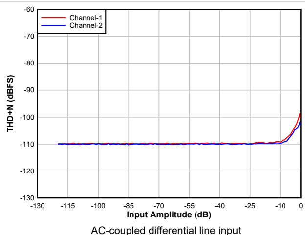
Figure 8-3. ADC THD+N Level vs Input
