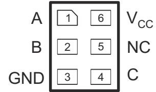
Figure 4-4. DSF Package 6-Pin X2SON (Top View)
