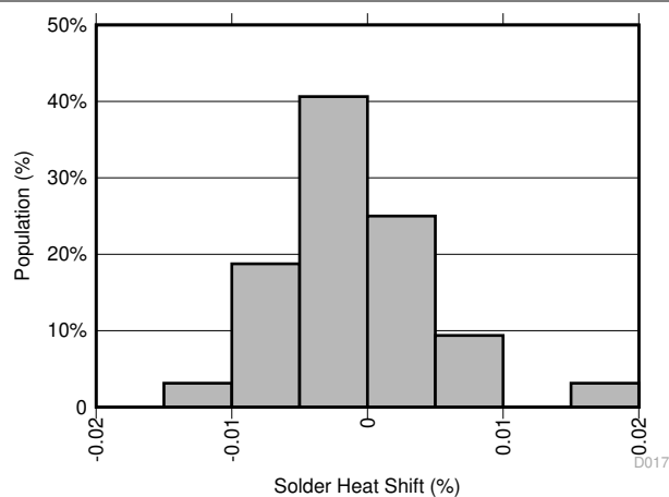
Figure 6-19. Solder Heat Shift Distribution
