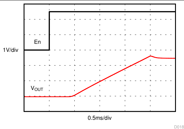
Figure 6-20. Turn-on Time (Enable)
