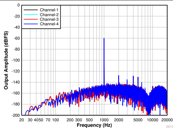
Figure 6-20. PDM Input FFT With a -60-dBr Input
