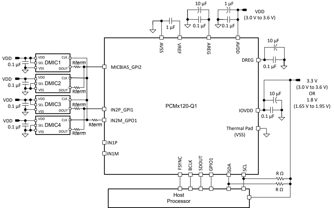
Figure 8-4. Four-Channel Digital PDM Microphone Recording Diagram
