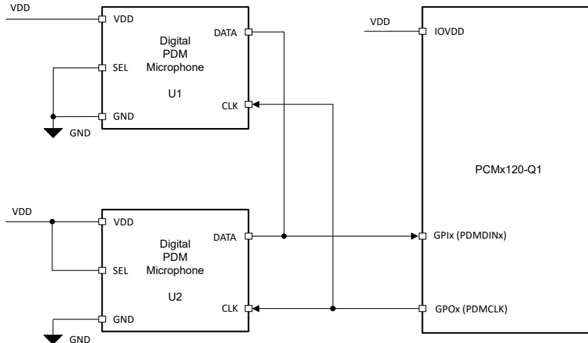
Figure 7-64. Digital PDM Microphones Connection Diagram for the PCM3120-Q1
