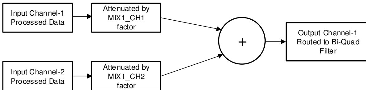
Figure 7-18. Programmable Digital Mixer Block Diagram
