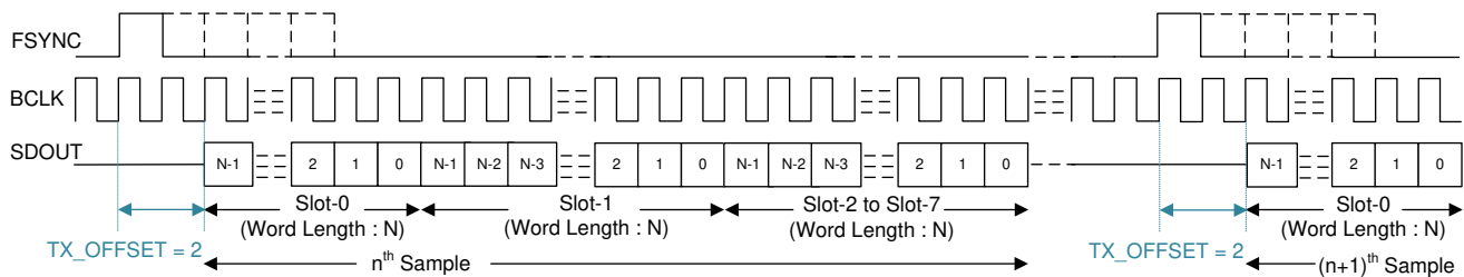
Figure 7-2. TDM Mode Protocol Timing (TX_OFFSET = 2)
