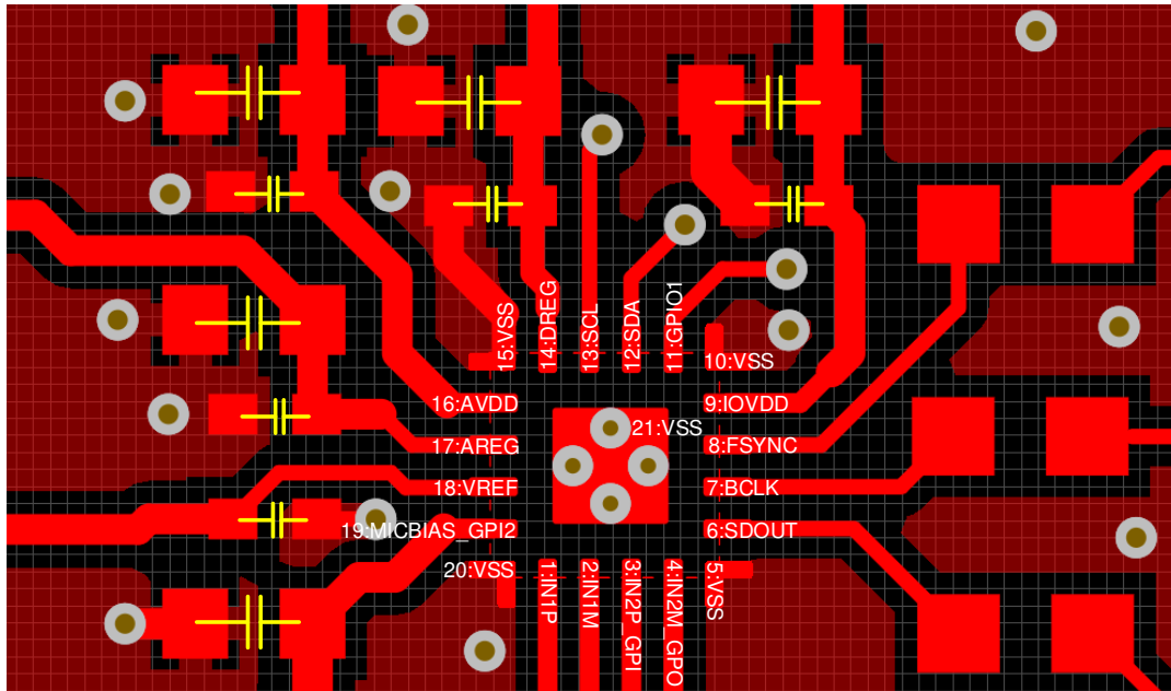
Figure 8-6. Layout Example
