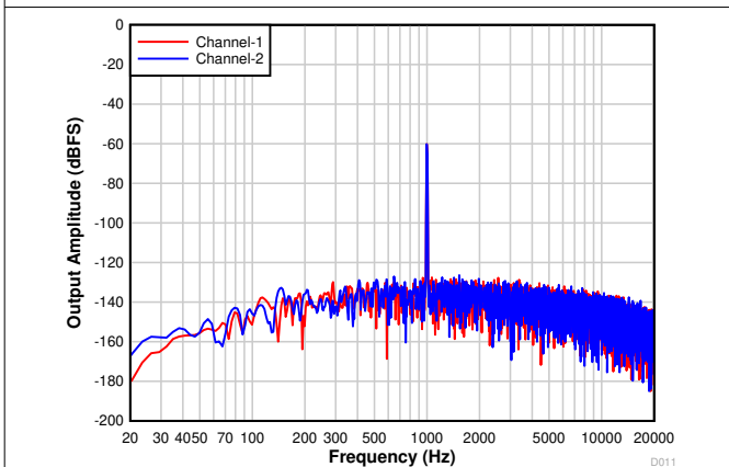
Figure 6-14. Differential FFT With a -60-dBr Input
