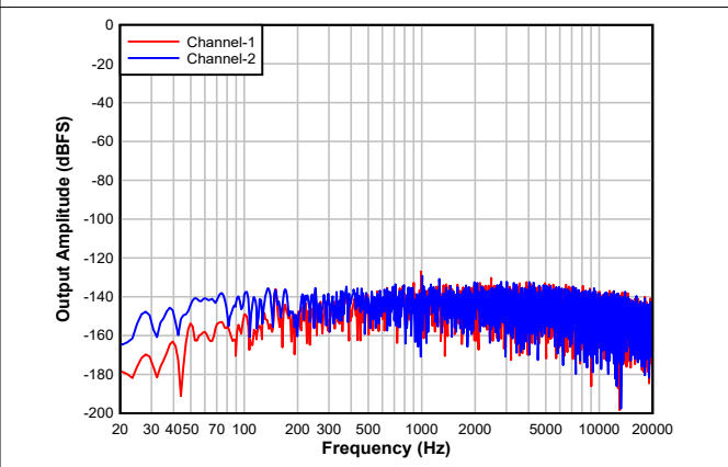
Figure 6-15. Single Ended FFT With Idle Input
