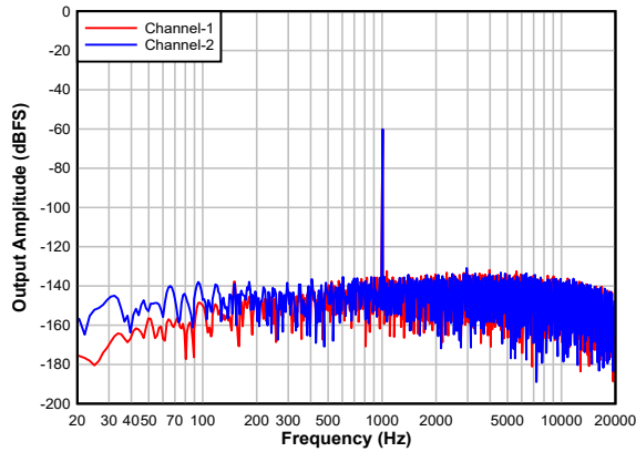
Figure 6-16. Single Ended FFT With a -60-dBr Input
