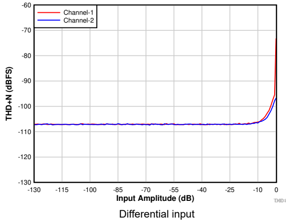
Figure 6-4. THD+N vs Input Amplitude
