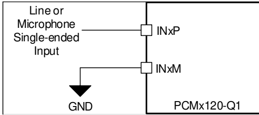
Figure 7-14. Single-Ended, DC-Coupled Input Connection
