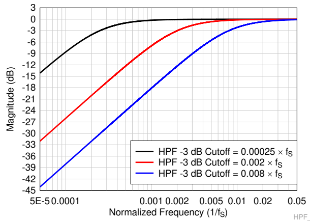
Figure 7-17. HPF Filter Frequency Response Plot
