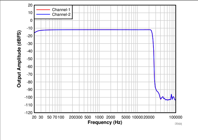
Figure 6-11. Frequency Response With a -12-dBr Input
