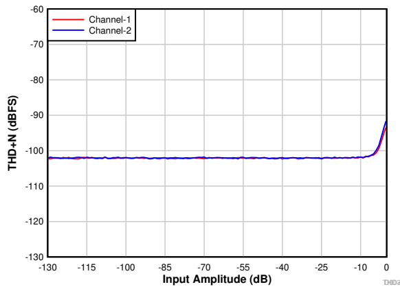
Figure 6-4. THD+N vs Input Amplitude
