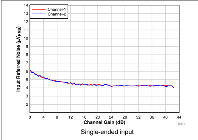
Figure 6-10. Input-Referred Noise vs Channel Gain
