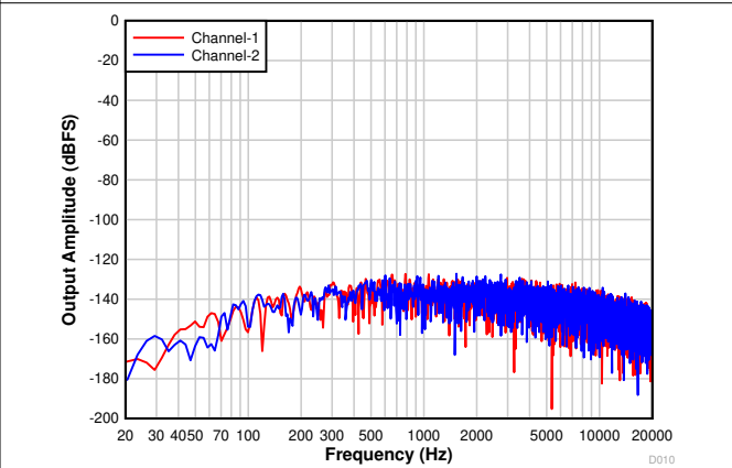
Figure 6-13. Differential FFT With Idle Input
