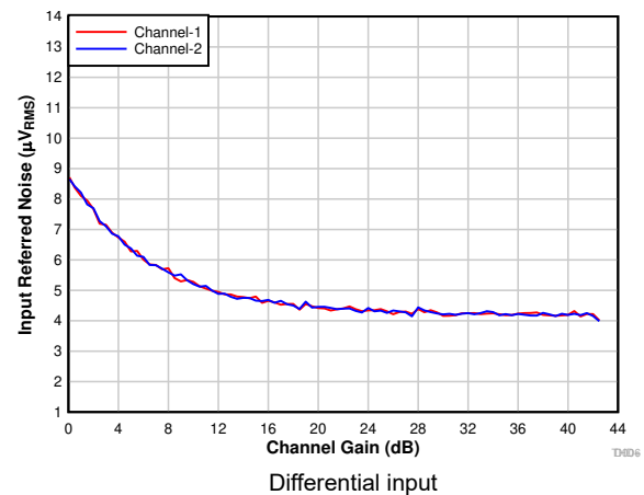
Figure 6-9. Input-Referred Noise vs Channel Gain
