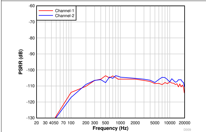
Figure 6-12. Power-Supply Rejection Ratio vs Ripple Frequency With 100-mV pp Amplitude
