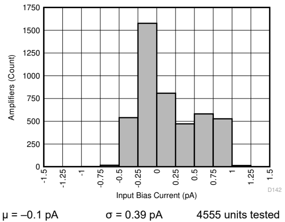
Figure 6-42. Input Bias Current Distribution
