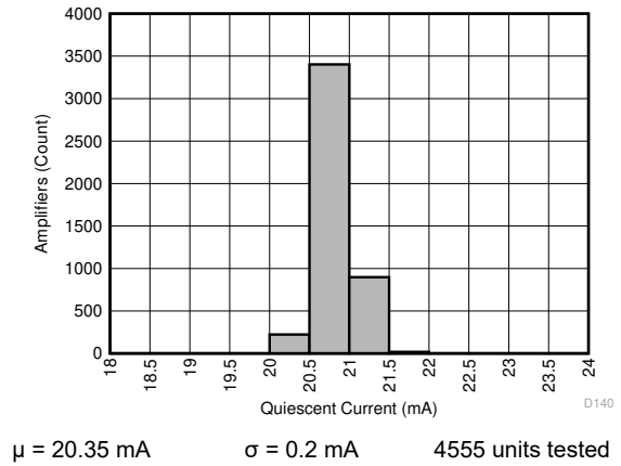
Figure 6-40. Quiescent Current Distribution
