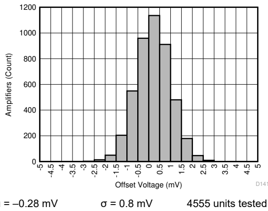
Figure 6-41. Offset Voltage Distribution
