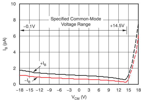
Figure 6-5. I_B vs Common-Mode Voltage
