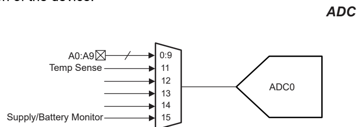
Figure 8-2. Analog Connections
