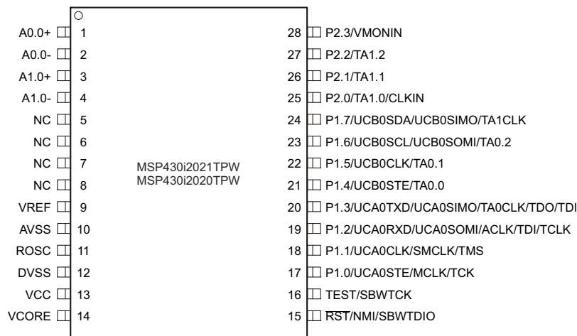
Figure 7-6. 28-Pin PW Package (Top View) – MSP430i2021, MSP430i2020
