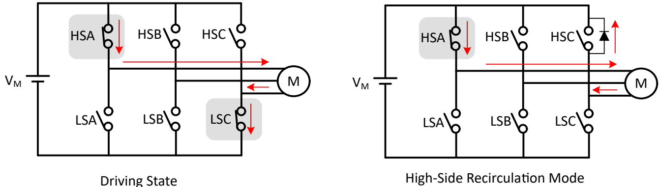
Figure 7-35. High-Side Recirculation
