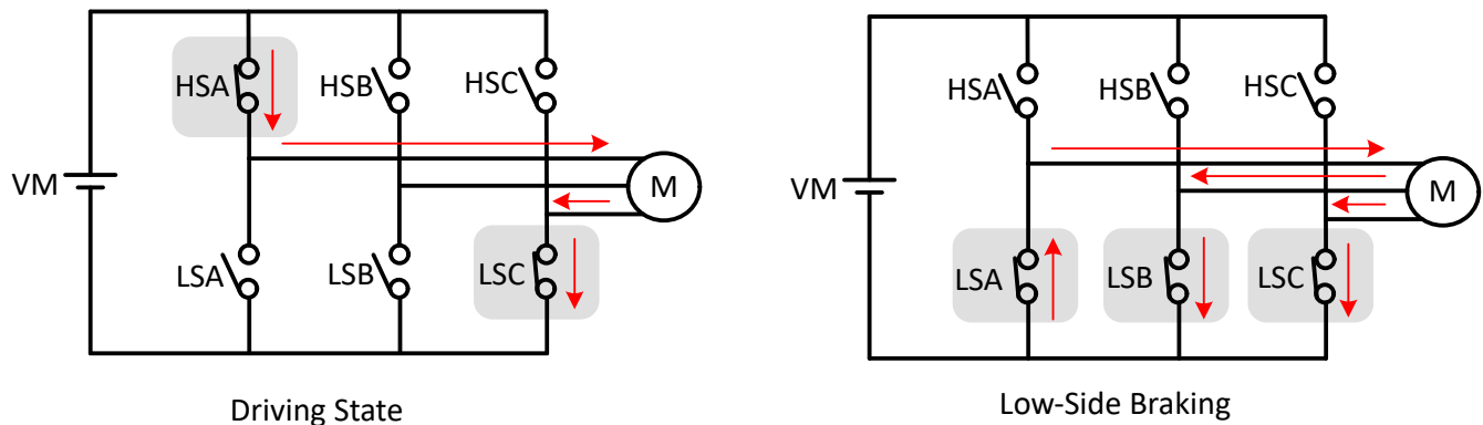
Figure 7-36. Low-Side Braking
