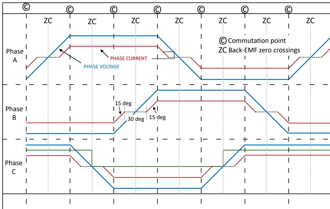
Figure 7-25. 150° commutation
