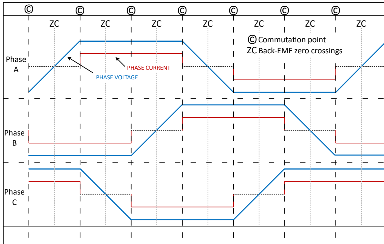
Figure 7-21. 120° commutation
