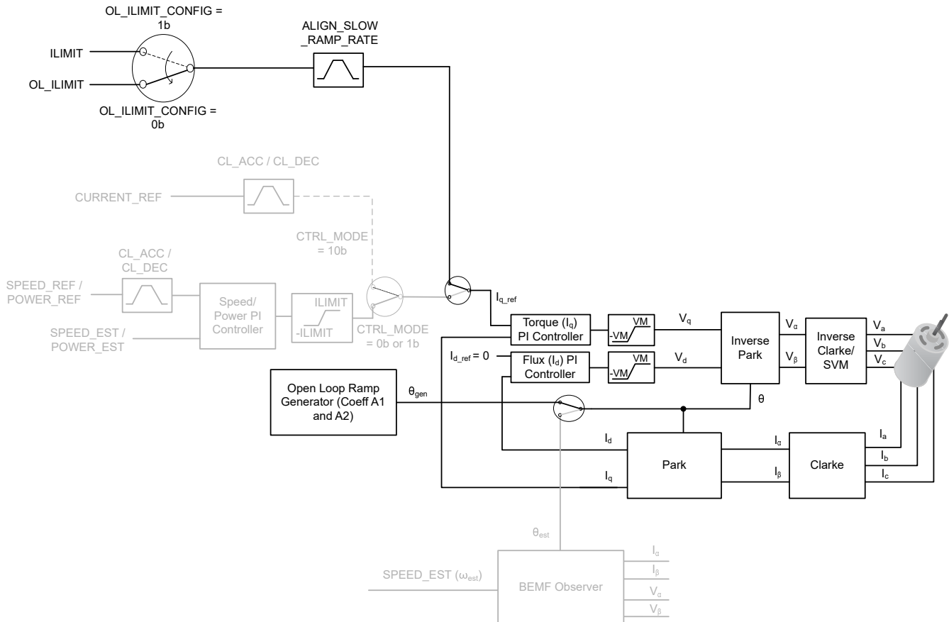
Figure 6-21. Open Loop
