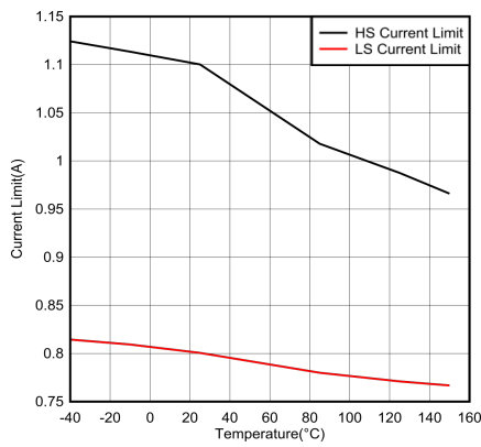
Figure 6-13. HS and LS Current Limit Versus Temperature- LMR54406
