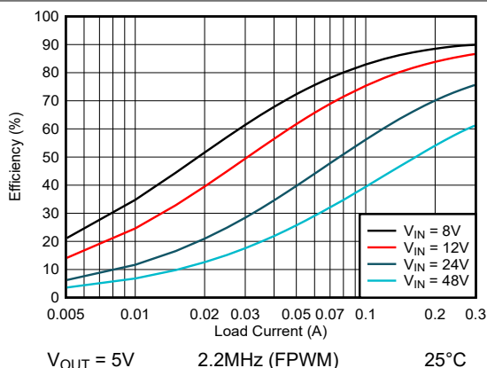
Figure 8-7. Efficiency
