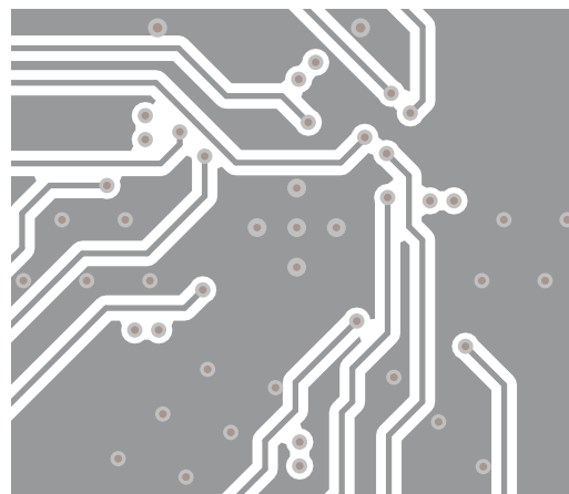
Figure 10-11. LMKDB1104 and LMKDB1104FS Layout Example - Bottom Layer
