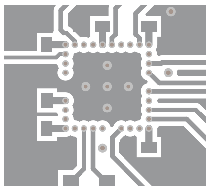
Figure 10-7. LMKDB1120 and LMKDB1120FS Layout Example - Bottom Layer
