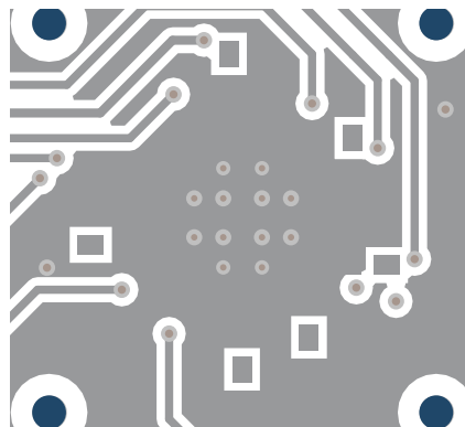
Figure 10-9. LMKDB1108 and LMKDB1108FS Layout Example - Bottom Layer
