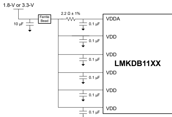
Figure 10-4. Power Supply Recommendation for LMKDB11XX Buffer
